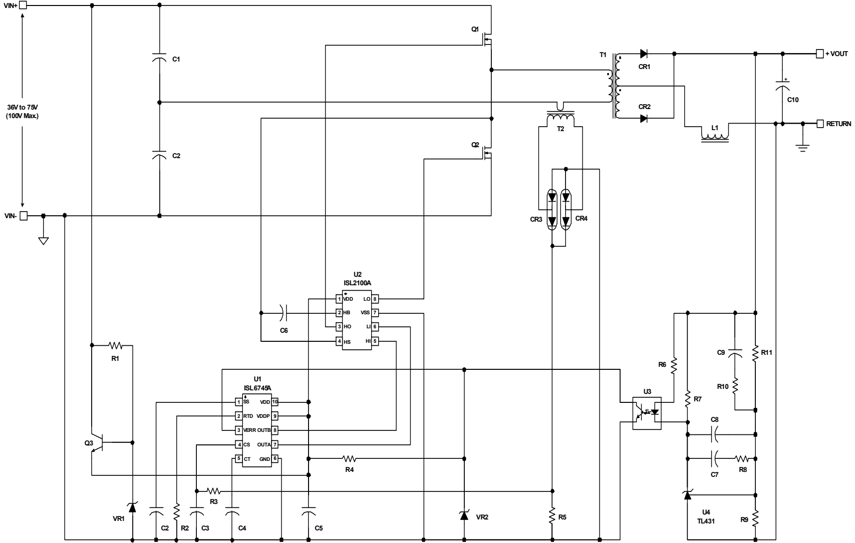
Figure 2. Typical Application
