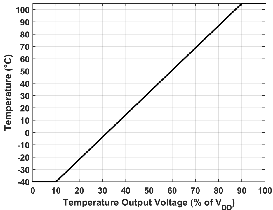
Figure 9. Temperature vs. VT Output Analog Voltage
