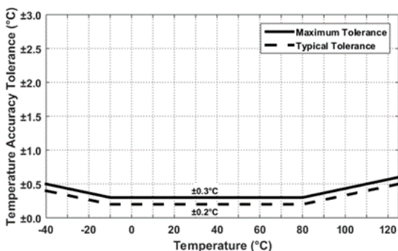
Figure 5. HS4111 Temperature Sensor Accuracy Tolerance
