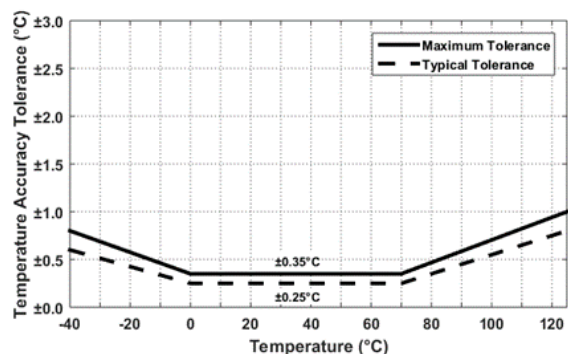
Figure 6. HS4113 Temperature Sensor Accuracy Tolerance
