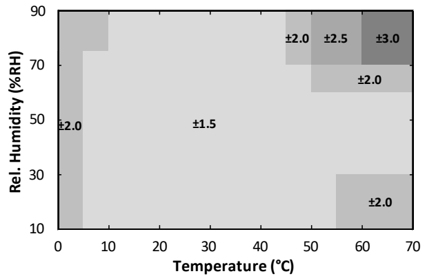
Figure 2. HS4111 RH Accuracy over Temperature
