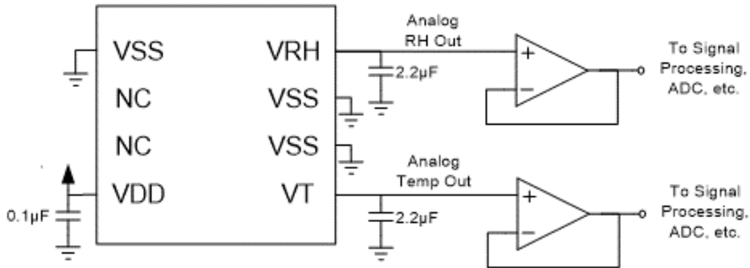
Figure 7. HS411x Application Circuit
