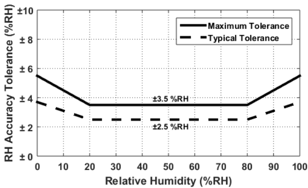
Figure 3. HS4113 RH Accuracy Tolerance at 25°C
