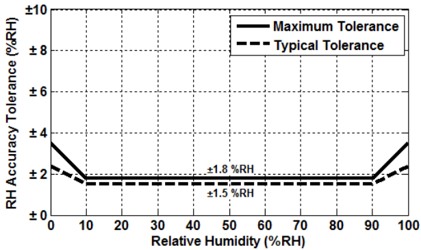
Figure 1. HS4111 RH Accuracy Tolerance at 25°C
