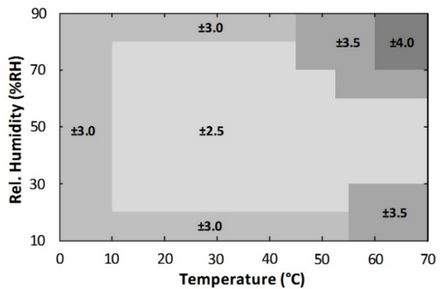
Figure 4. HS4113 RH Accuracy over Temperature
