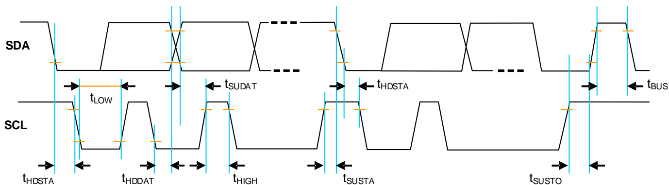
Figure 11. Timing Diagram
