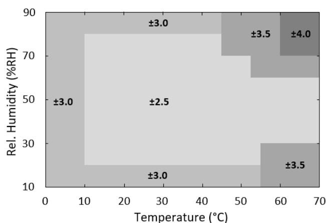
Figure 6. HS40x3 RH Accuracy over Temperature
