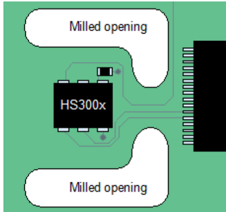
Figure 12. Milled PCB Openings for Thermal Isolation
