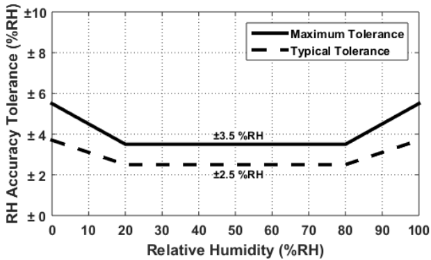
Figure 4. HS3103-ML1 RH Accuracy Tolerance at 25°C
