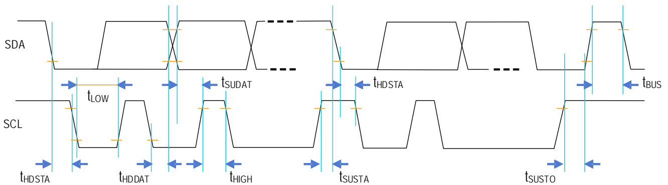
Figure 10. Timing Diagram
