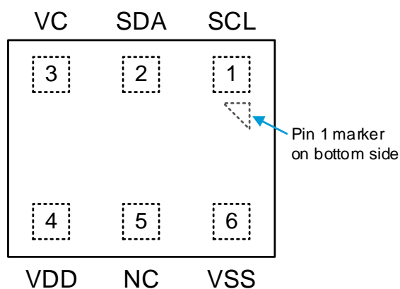
Figure 1. Pin Assignments for 3mm x 2.41mm 6-LGA Package – Top View
