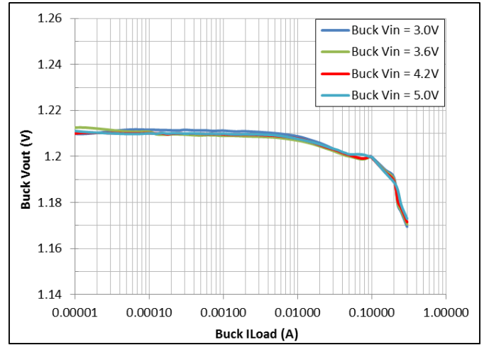
Figure 24: Buck V_{OUT} = 1.2 V
