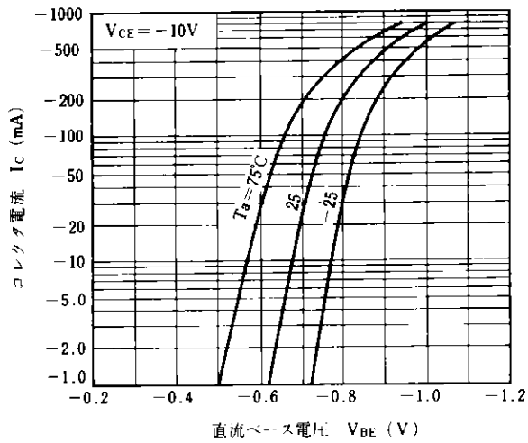
COLLECTOR CURRENT vs. BASE TO EMITTER VOLTAGE
