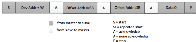
Figure 1. Single-Byte Write
