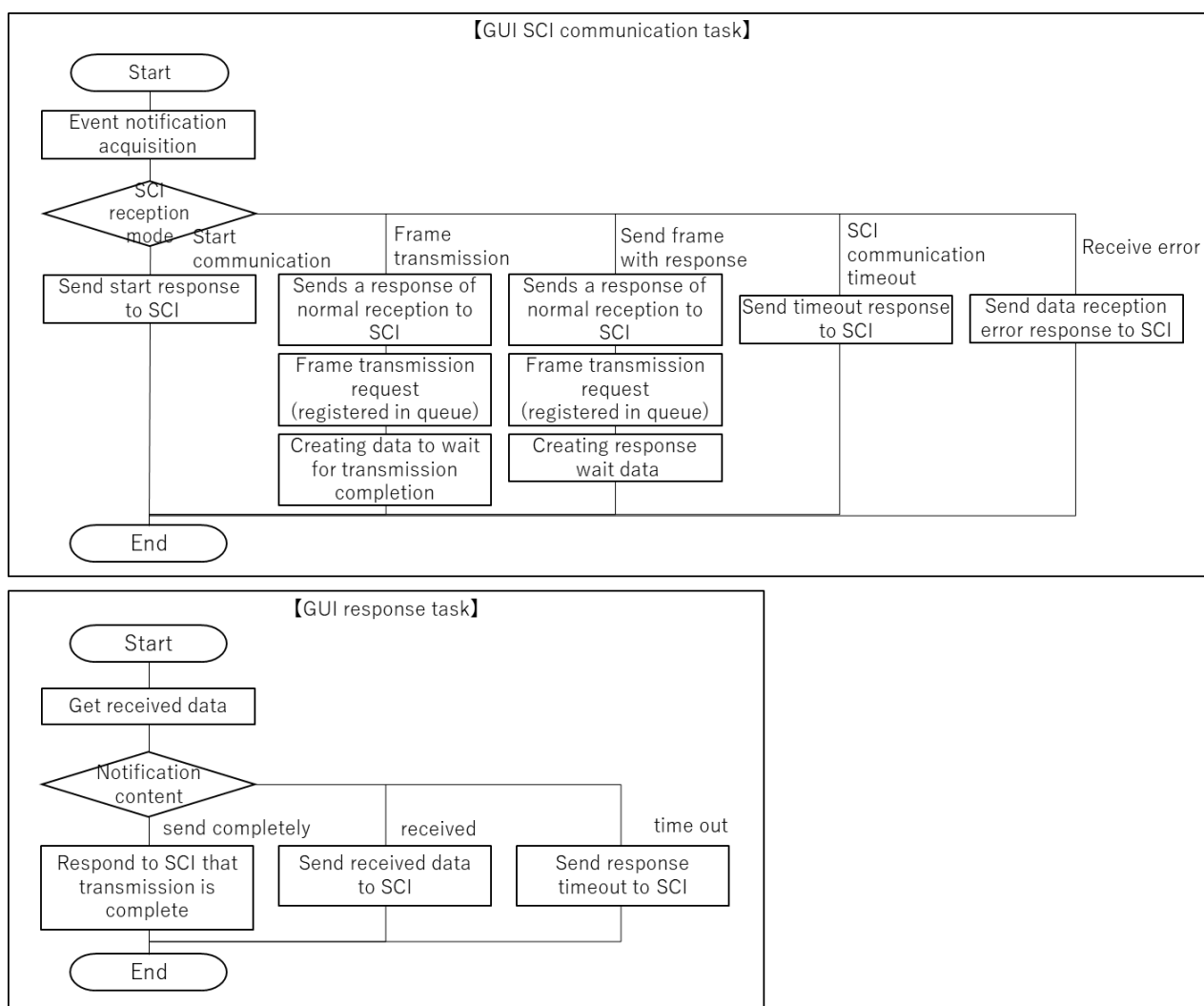
Figure 42 GUI application task flow diagram
