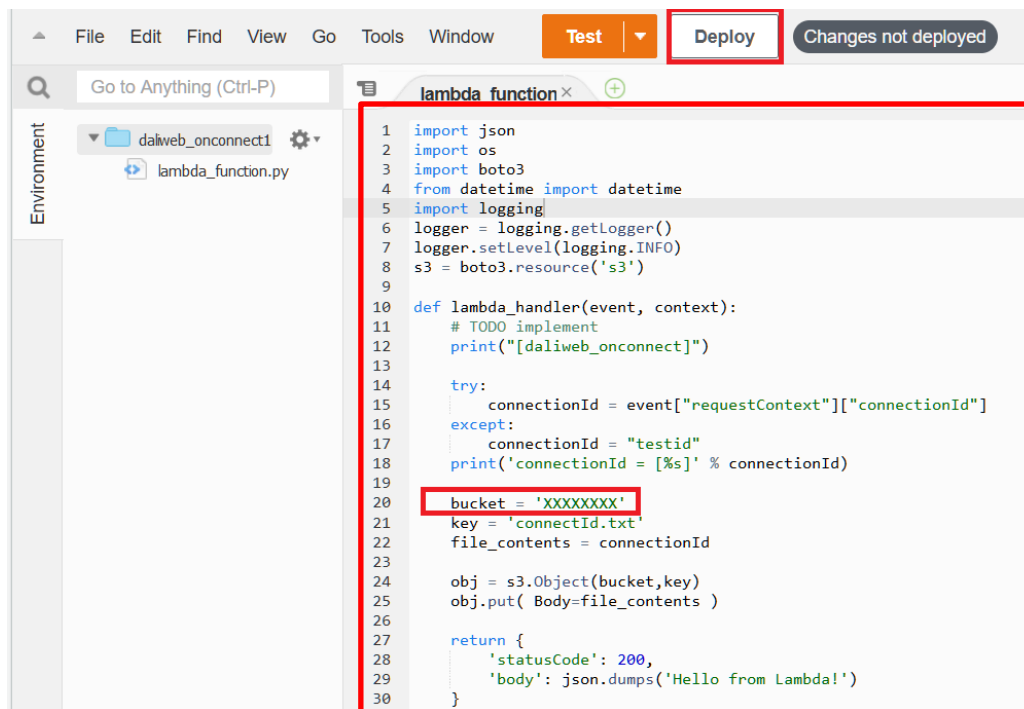
Figure 84 lambda (3/6)
