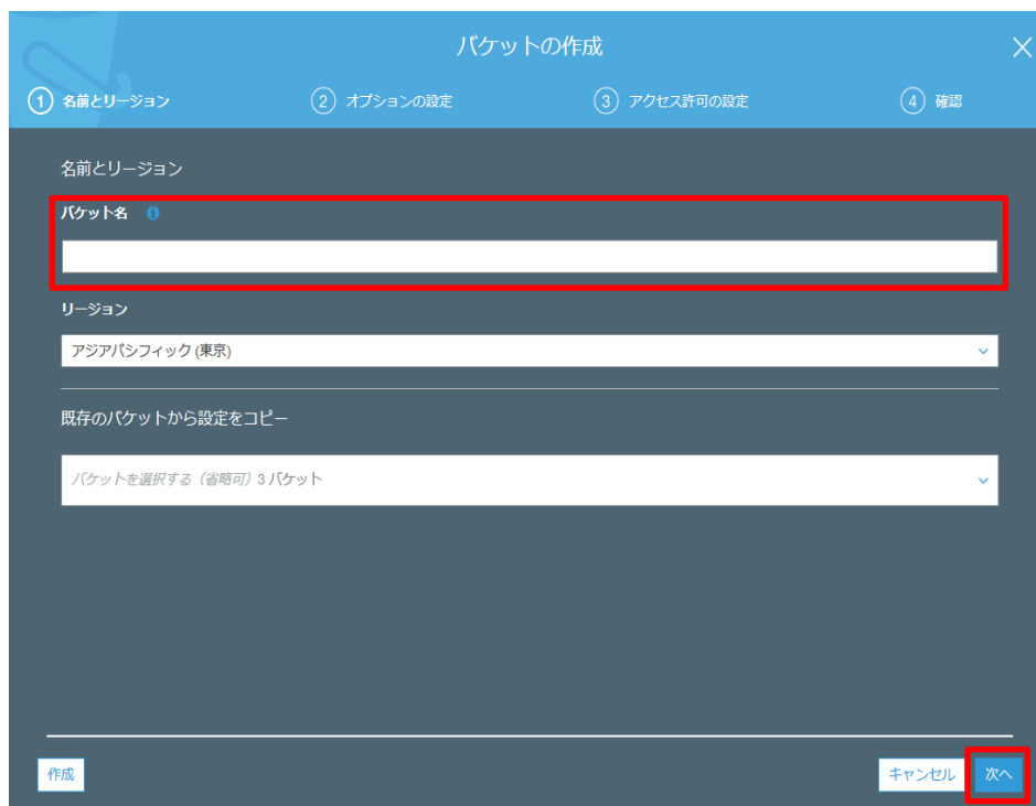
Figure 74 Amazon S3 (2/9)
