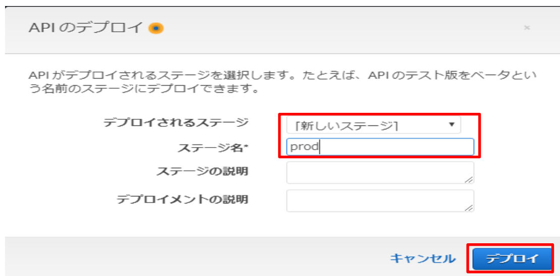
Figure 96 API Gateway (9/15)
