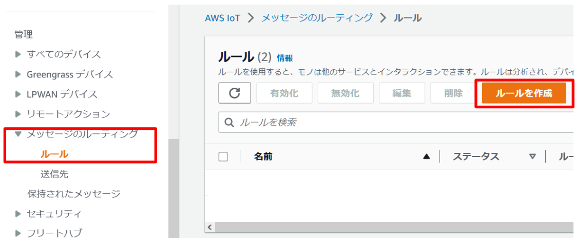
Figure 103 Aws IoT (1/7)
