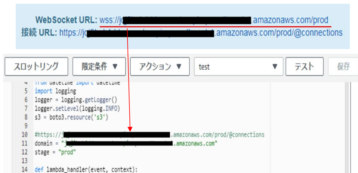
Figure 99 API Gateway (12/15)
