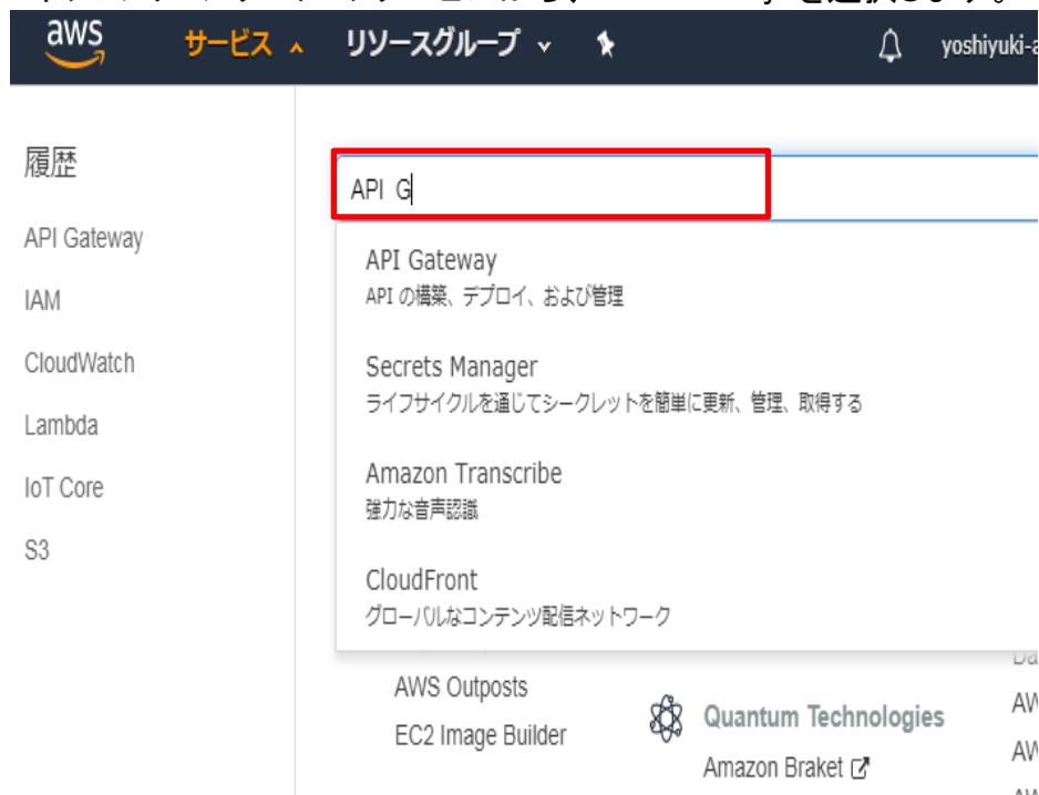
Figure 88 API Gateway (1/15)
