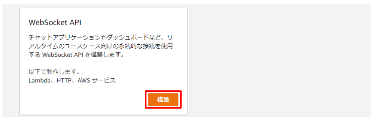
Figure 90 API Gateway (3/15)
