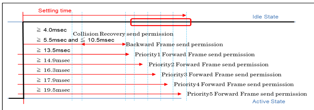
Figure 15 Collision avoidance transmission timing
