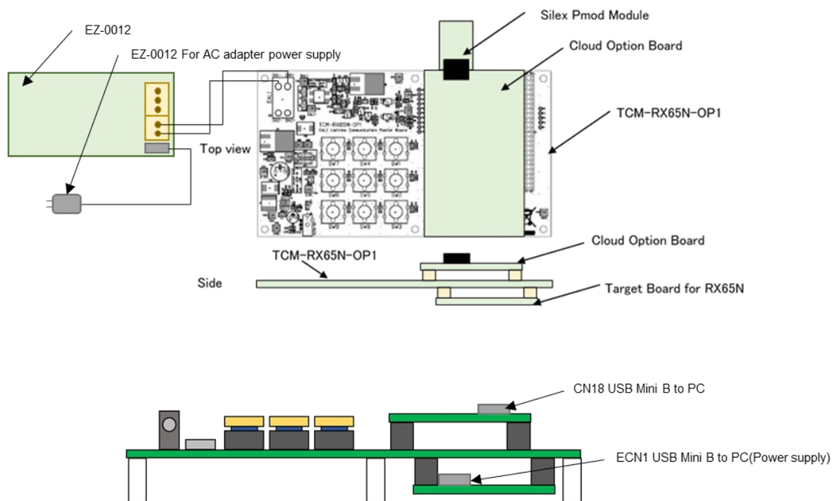
Figure 51 Overall hardware configuration diagram
