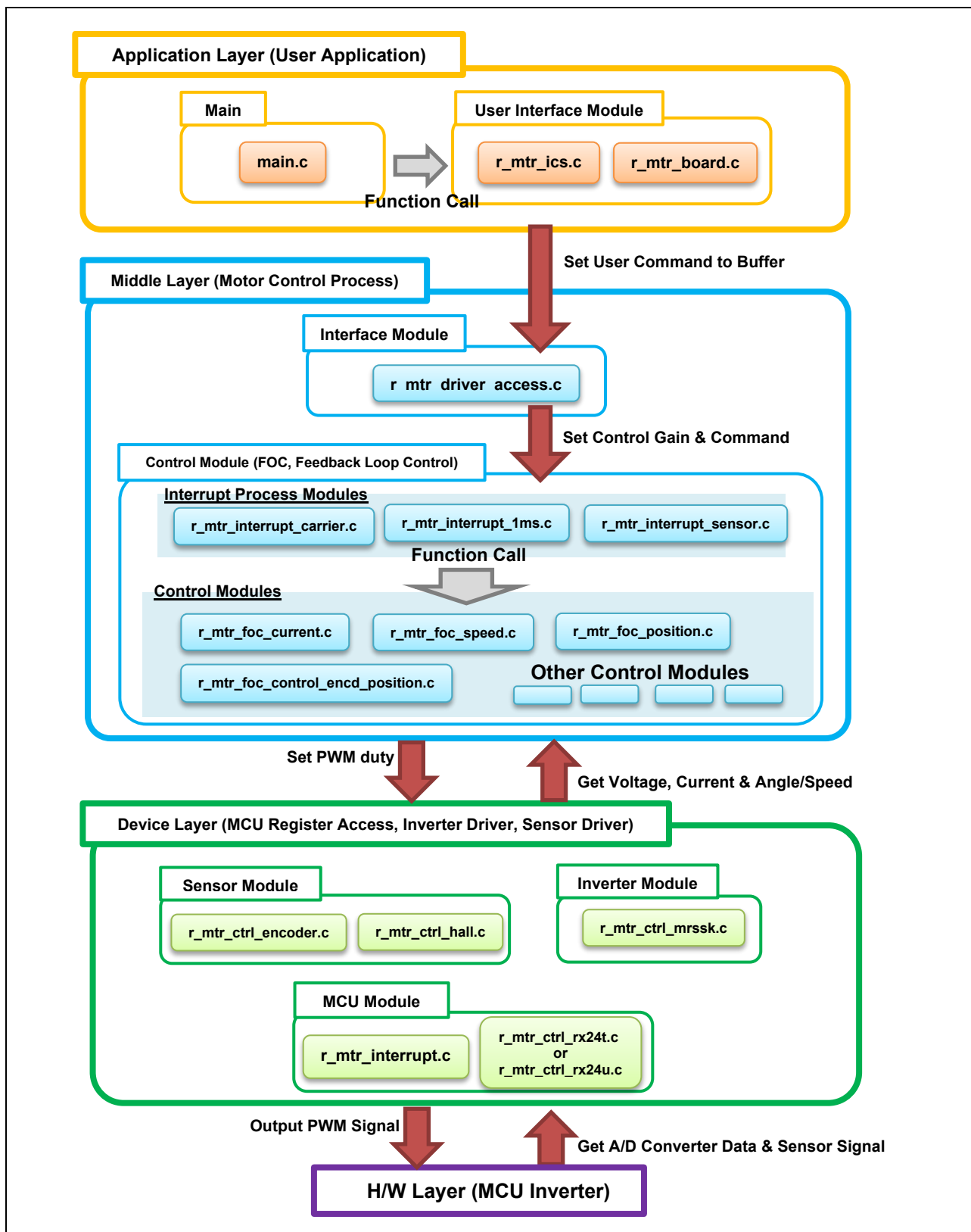
Figure 2-4 Module Configuration
