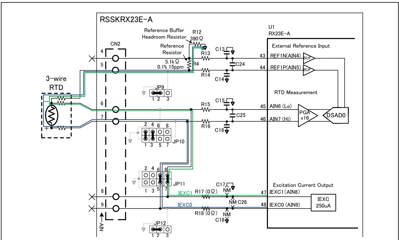
Figure 4-2 Temperature Measurement System with a 3-Wire RTD
