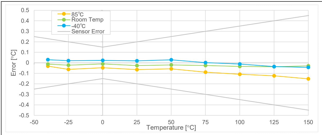
Figure 7-2 4-wire RTD Temperature Measurement Error
