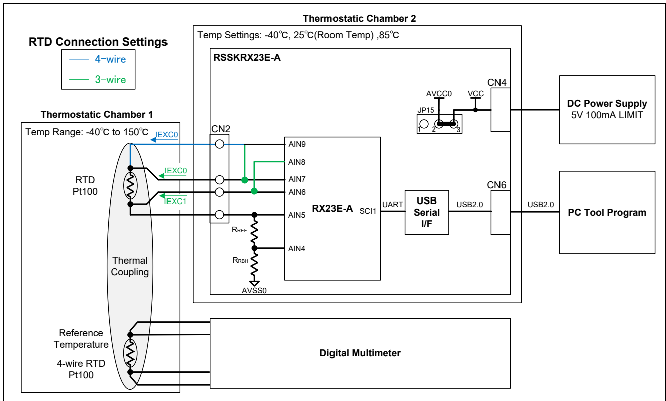
Figure 7-1 Configuration of Temperature Measurement by RTD
