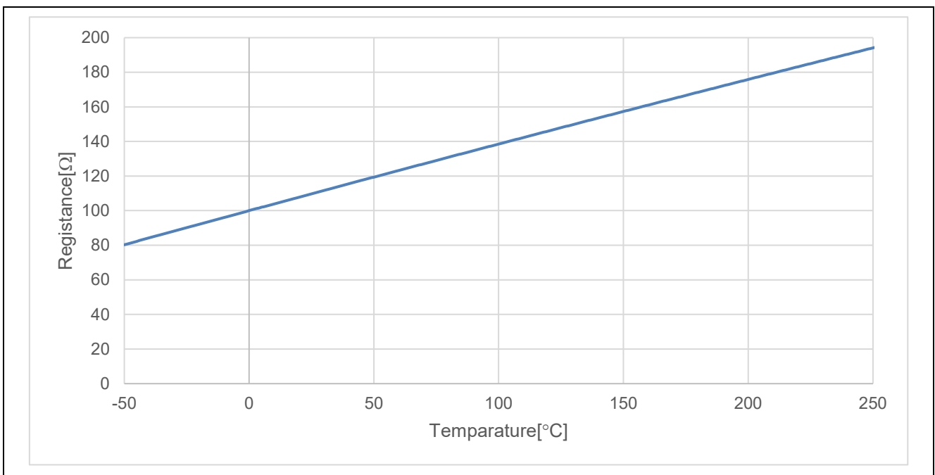
Figure 4-4 Temperature vs. Resistance Value of a Pt100Ω Platinum Resistance Temperature Detector (from IEC 60751)
