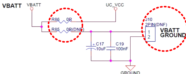
Figure 2.3 VBATT Circuit Detail Excerpted from RSKRX231 CPU Board Schematics
