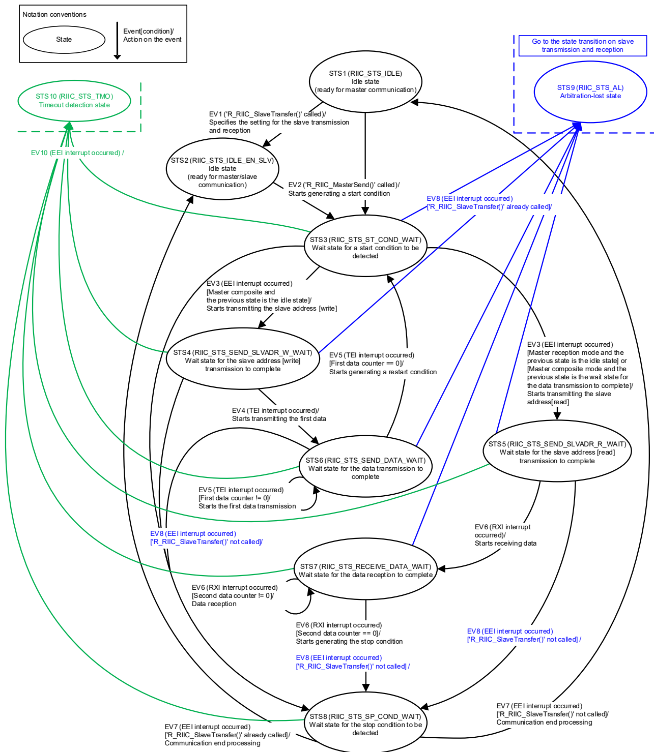
Figure 6.3 State Transition on Master Reception (R_RIIC_MasterReceive() Called)
