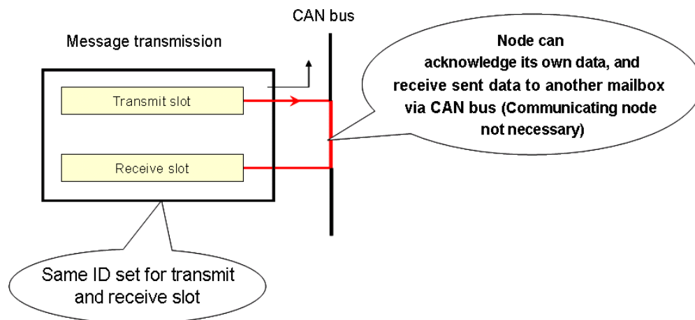
Figure 7. External Loopback.
