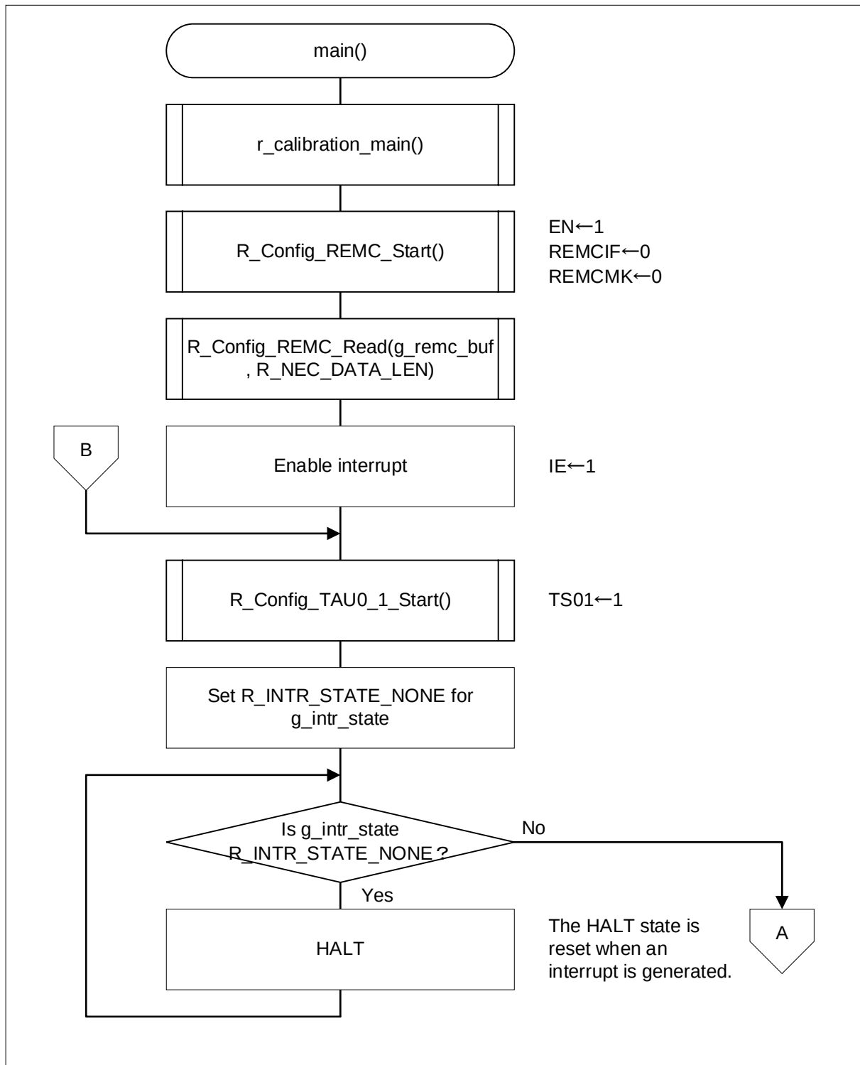
Figure 4-1 Main Processing (1/2)
