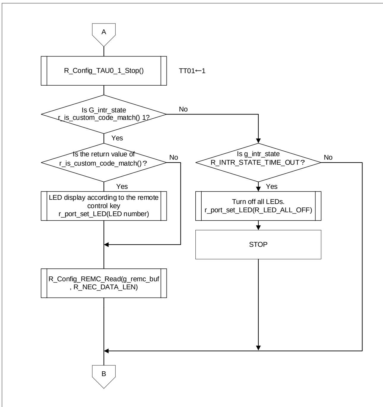
Figure 4-2 Main Processing (2/2)
