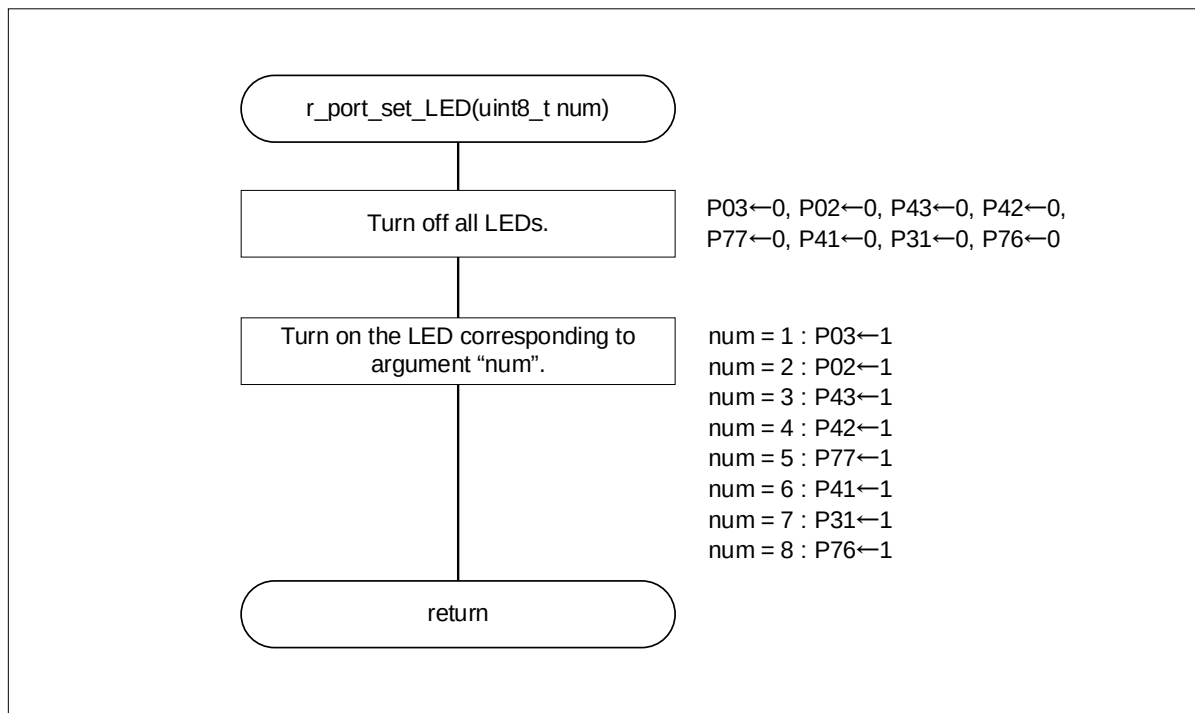
Figure 4-8 LED Lighting Control
