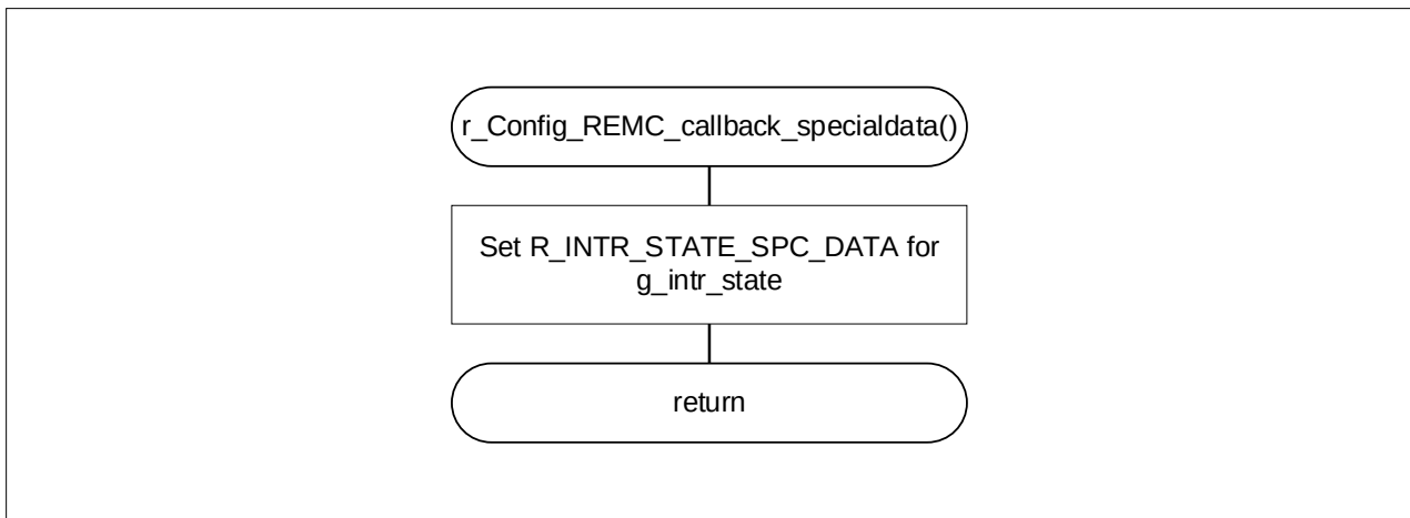
Figure 4-6 REMC Special Data Pattern Match Interrupts
