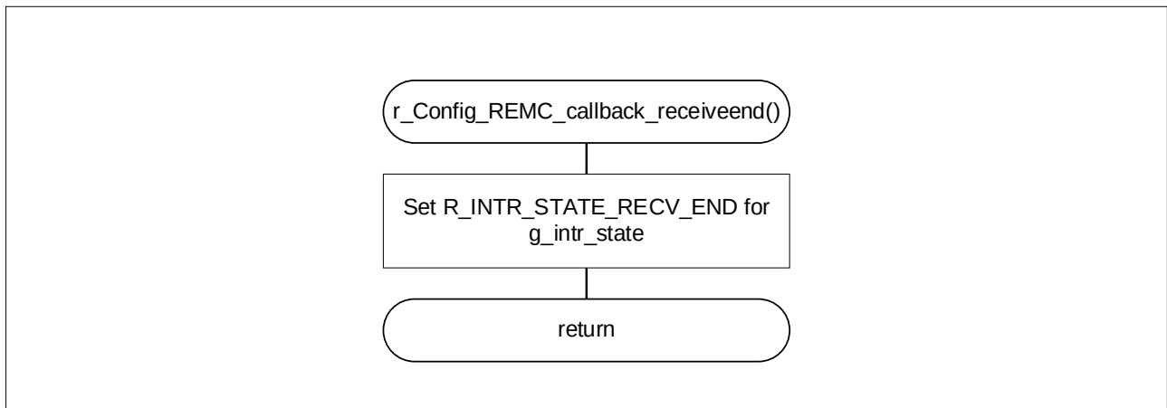
Figure 4-4 REMC Reception Complete Interrupts
