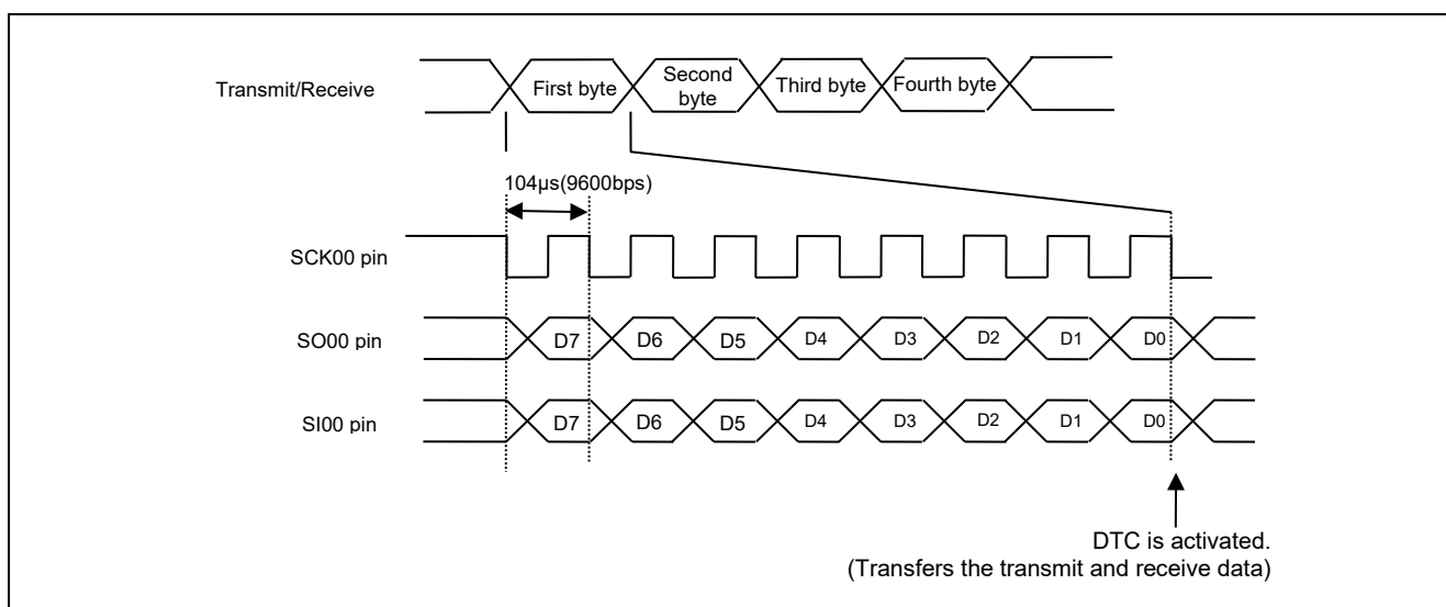
Figure 1.1 Timing and Communication Format (Transmitting/Receiving data is 4 bytes)
