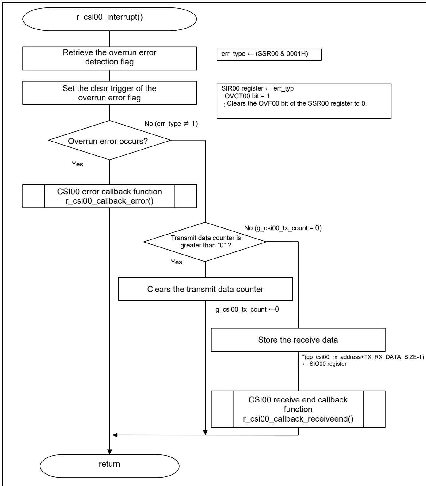
Figure 5.19 CSI00 Transfer End Interrupt
