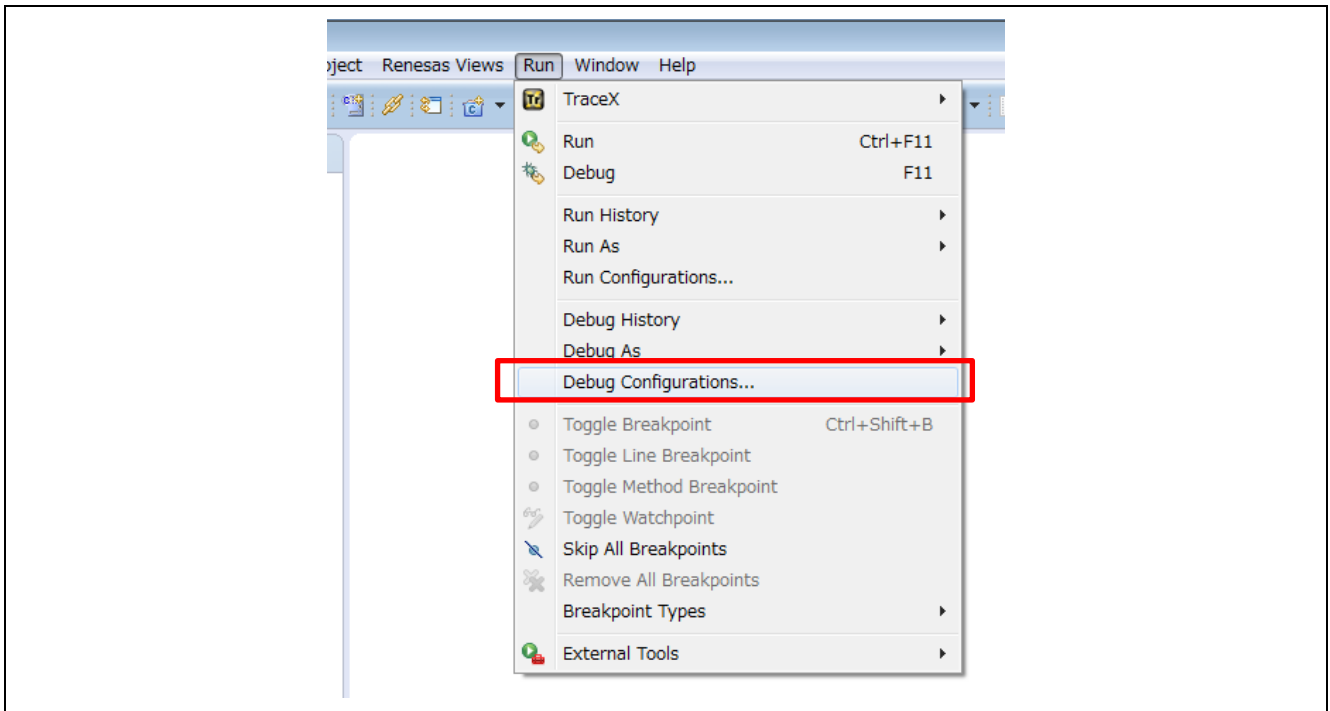
图9 “Run” 菜单
