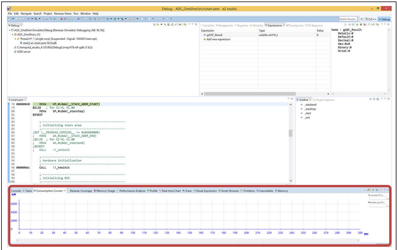
图 7 “Consumption Current” 栏
