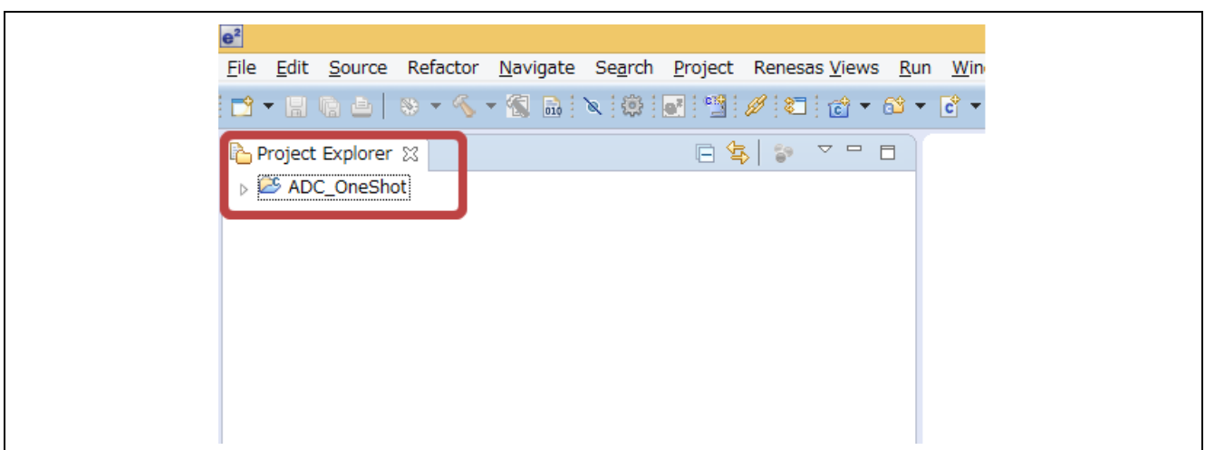
图4 Project Explorer
