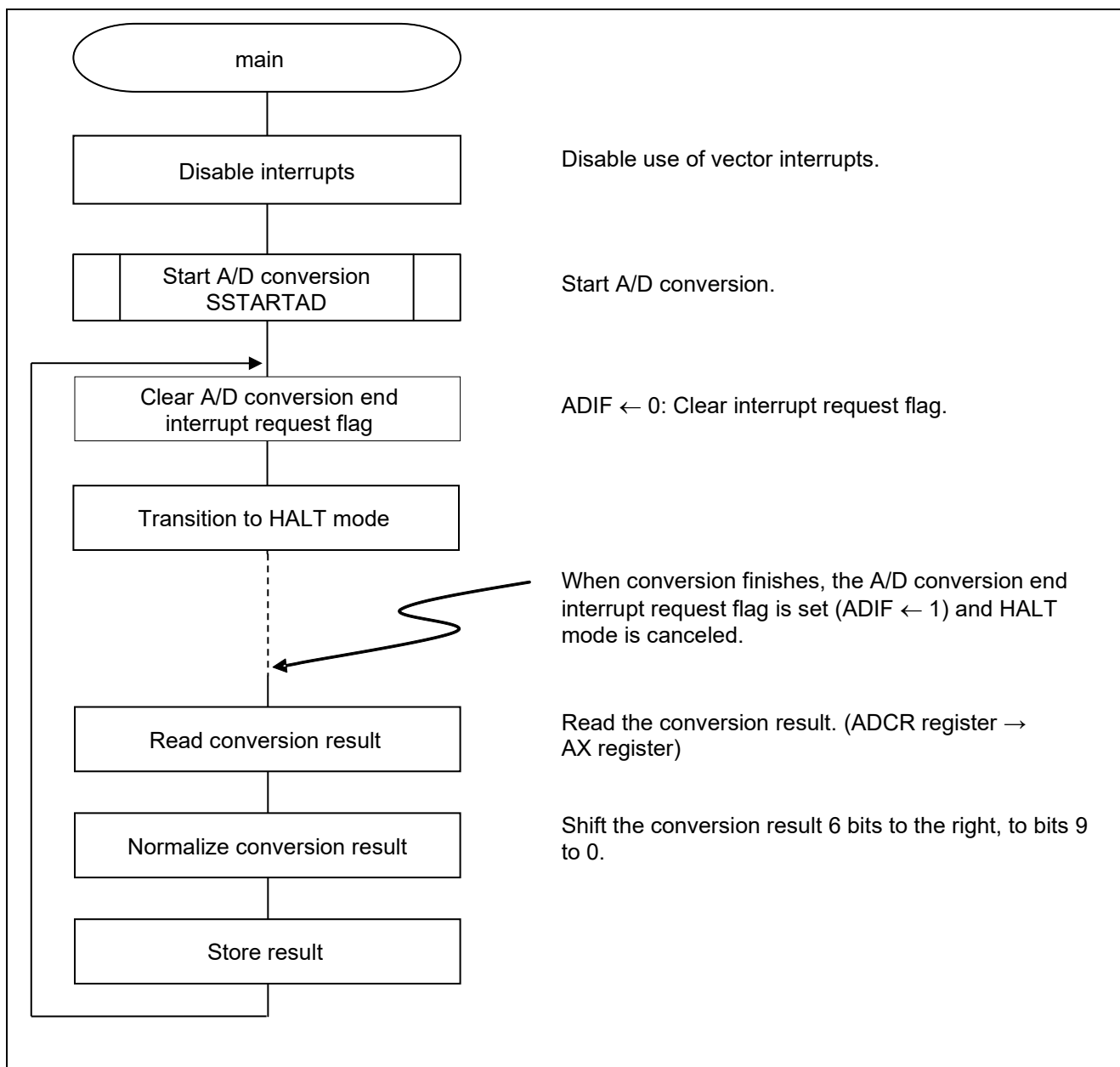
Figure 5.6 Main Processing
