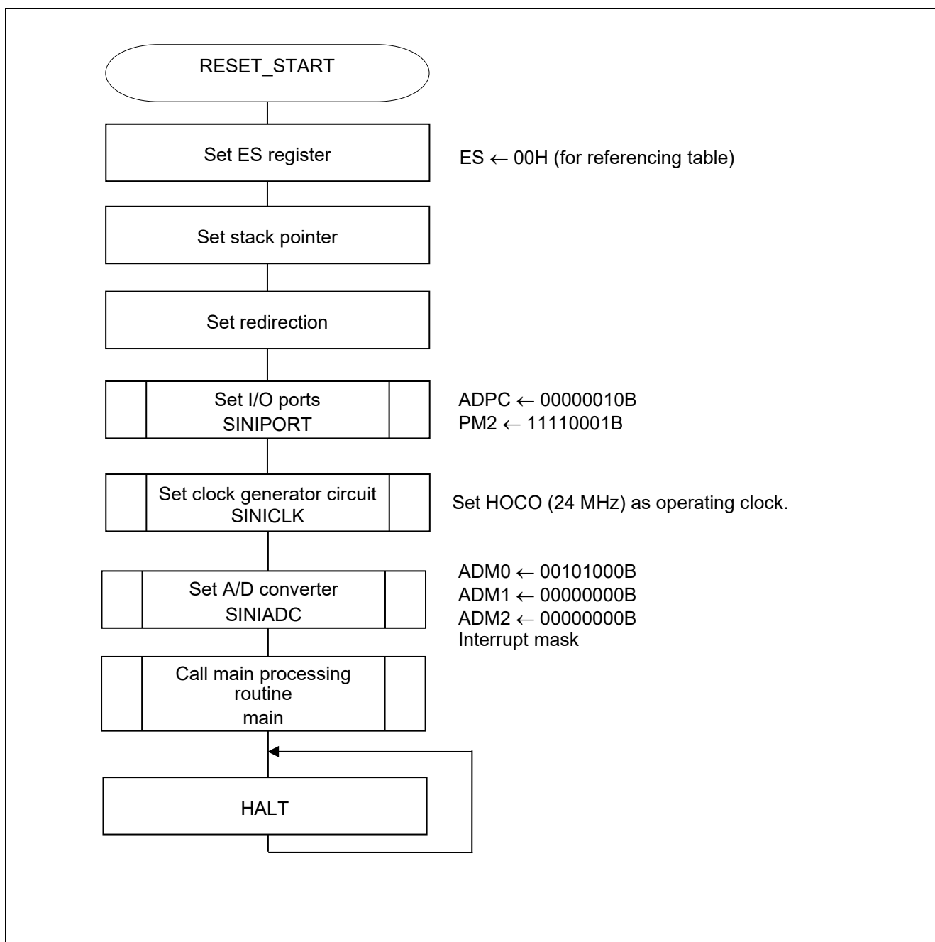
Figure 5.2 CPU Initialization
