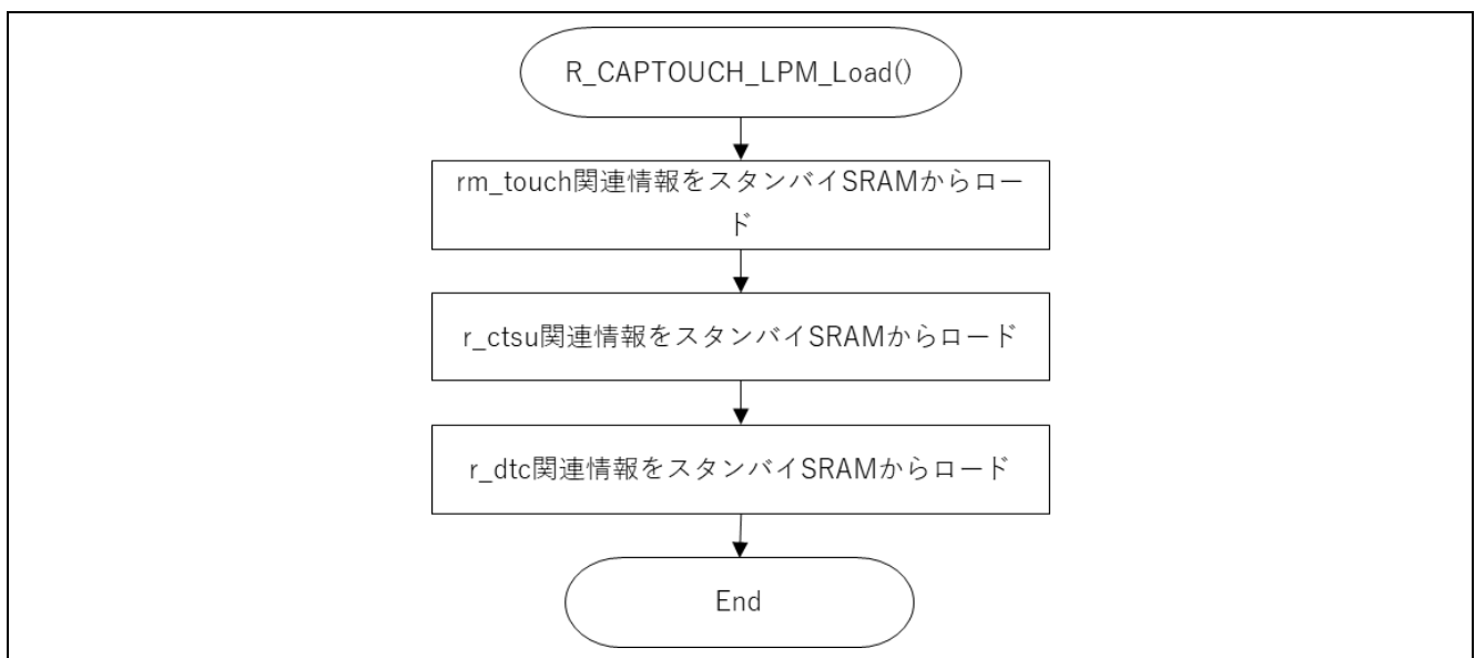
図 4-10 R_CAPTOUCH_LPM_Load ()
