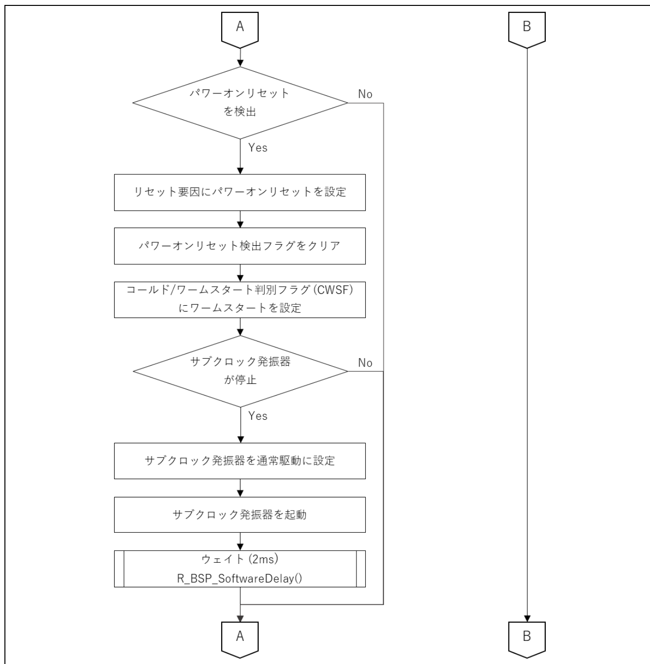
図 4-6 R_BSP_WarmStart () (2/4)
