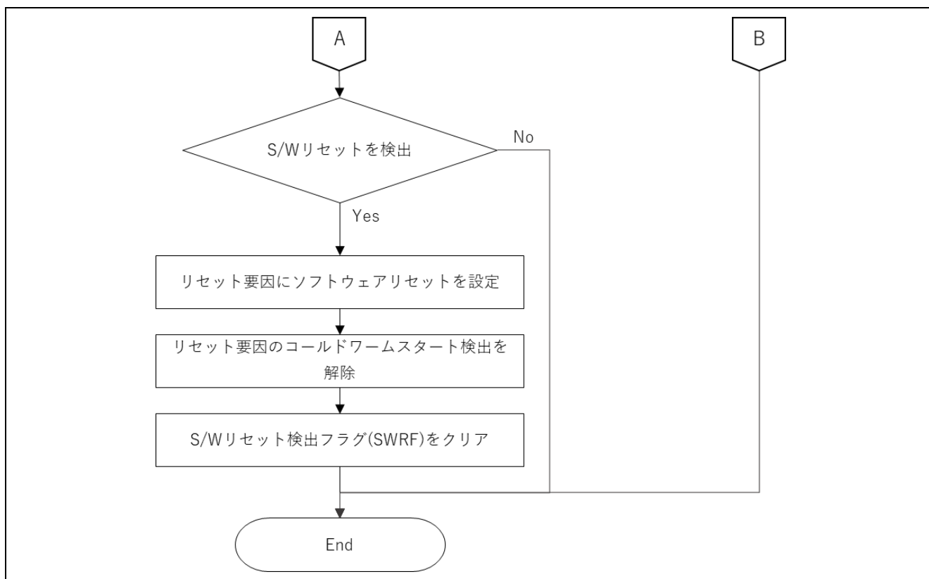
図 4-8 R_BSP_WarmStart () (4/4)
