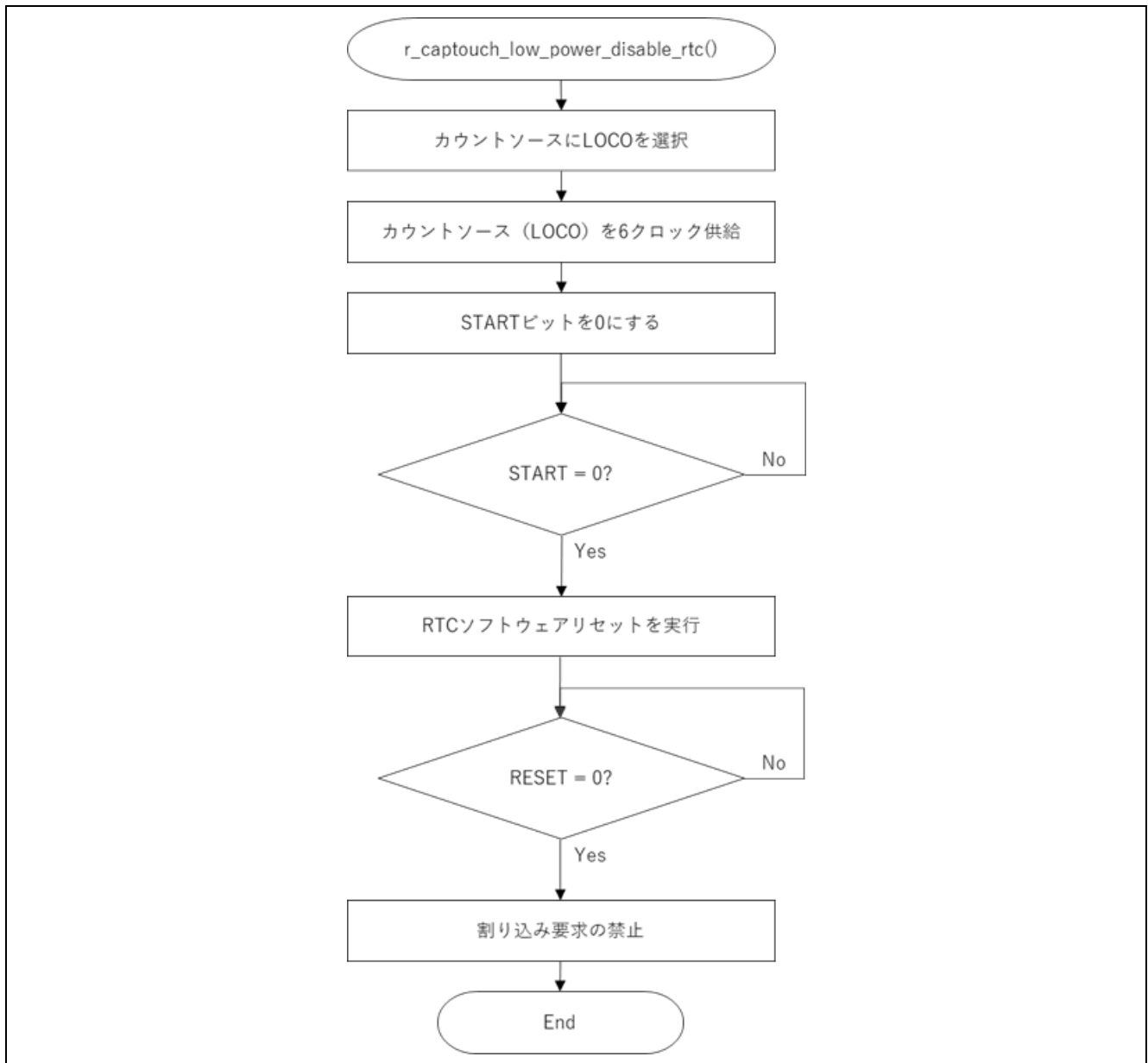
図 4-4 r_captouch_low_power_disable_rtc ()
