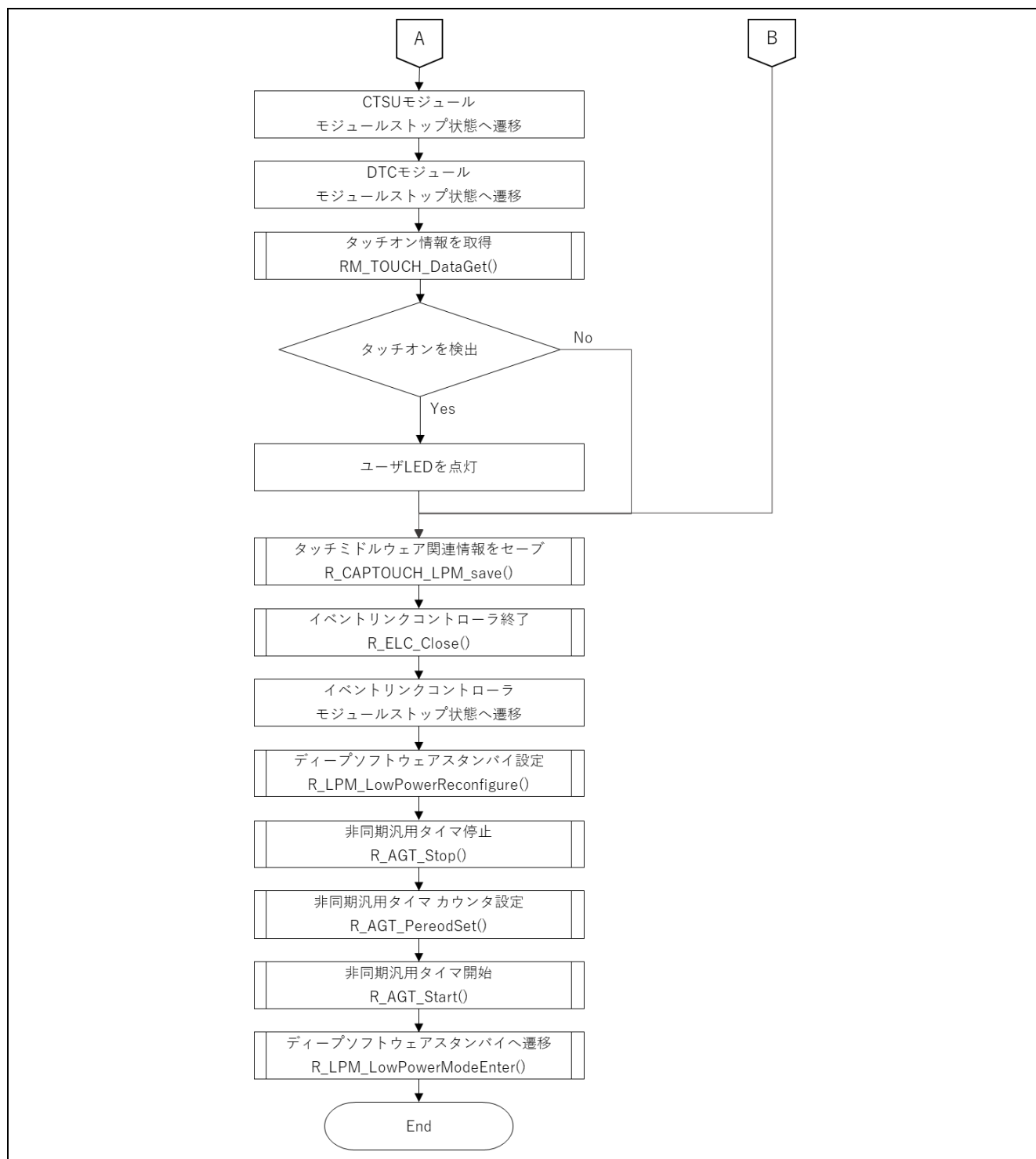
図 4-2 qe_touch_main () (2/2)
