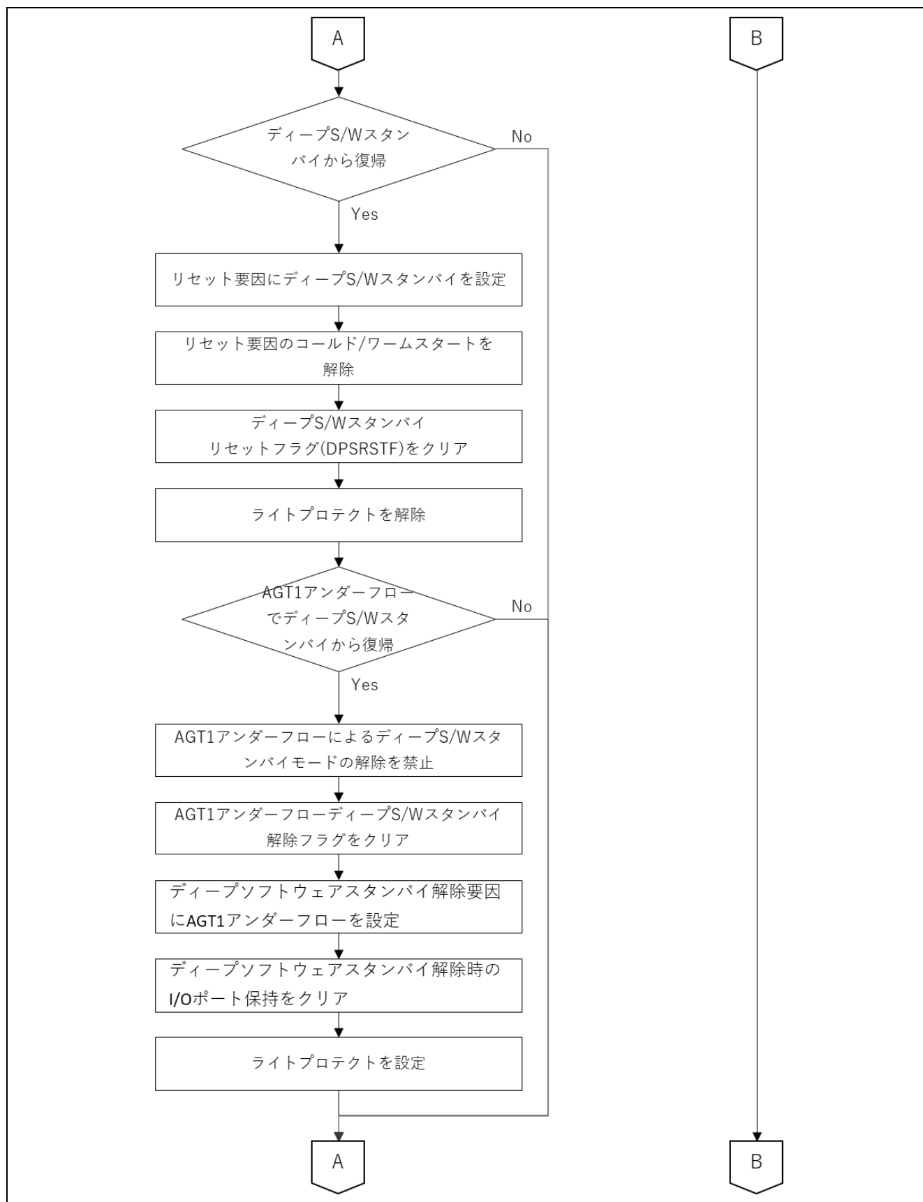
図 4-7 R_BSP_WarmStart () (3/4)
