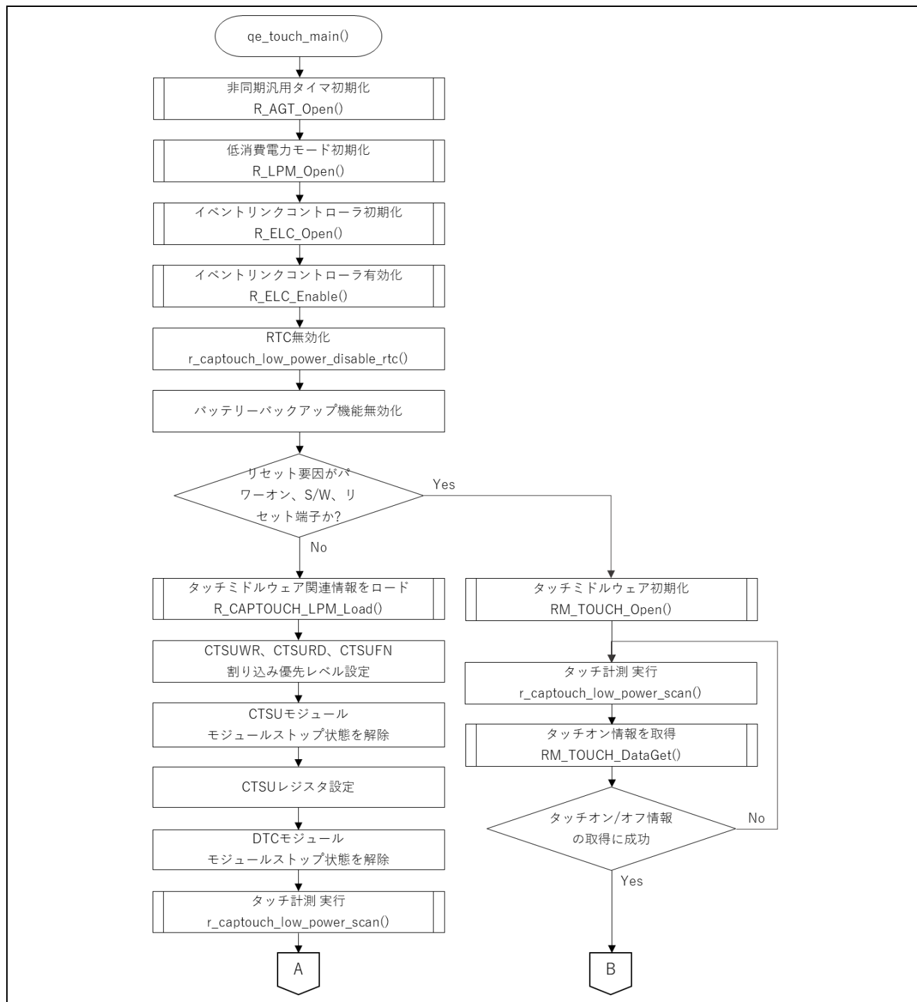
図 4-1 qe_touch_main () (1/2)
