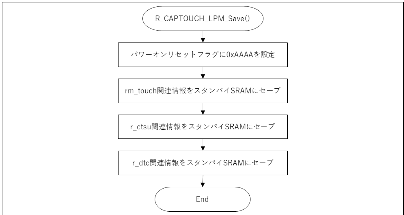
図 4-9 R_CAPTOUCH_LPM_Save ()
