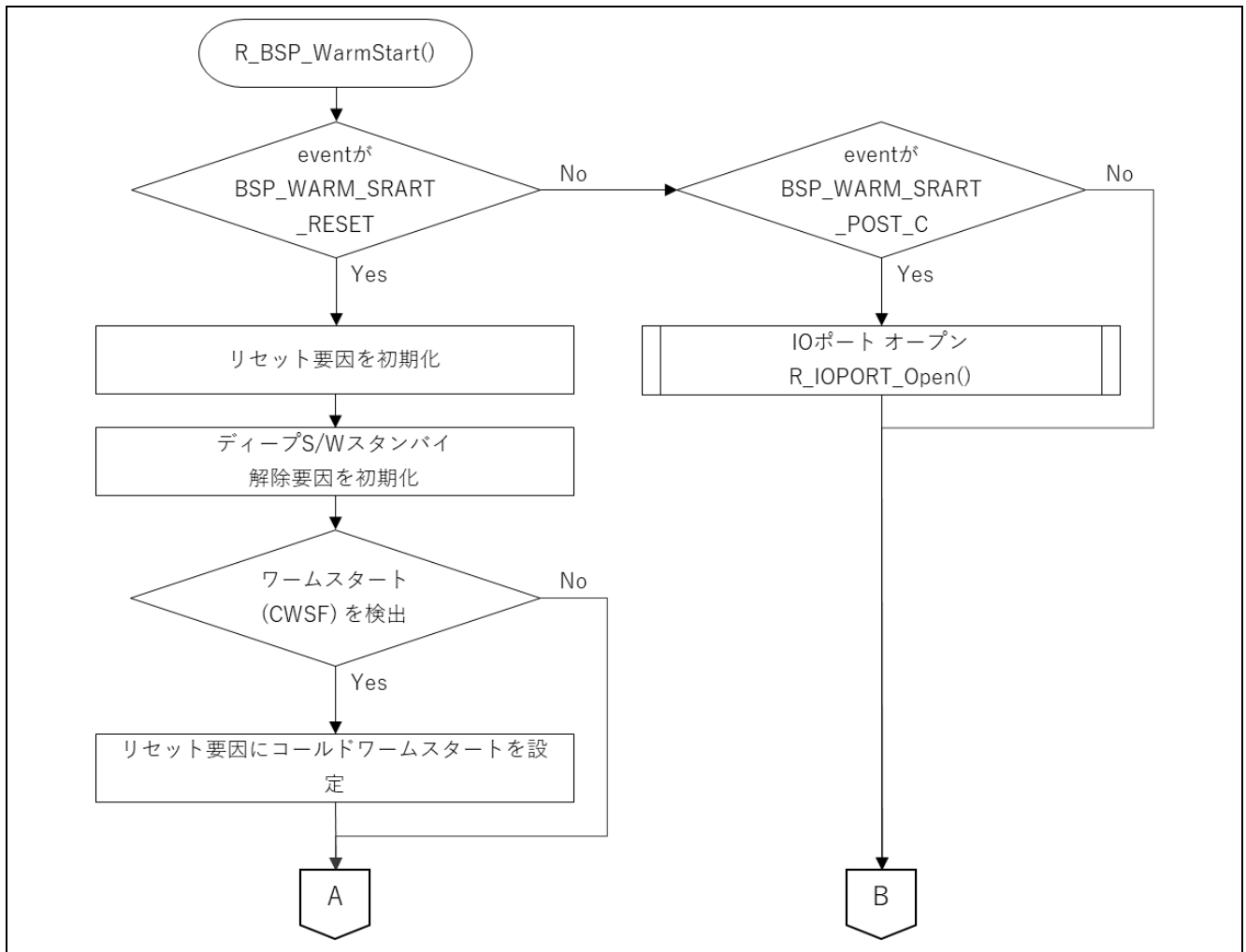
図 4-5 R_BSP_WarmStart () (1/4)
