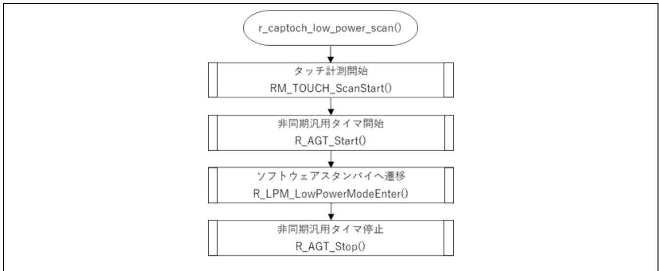
図 4-3 r_captouch_low_power_scan ()
