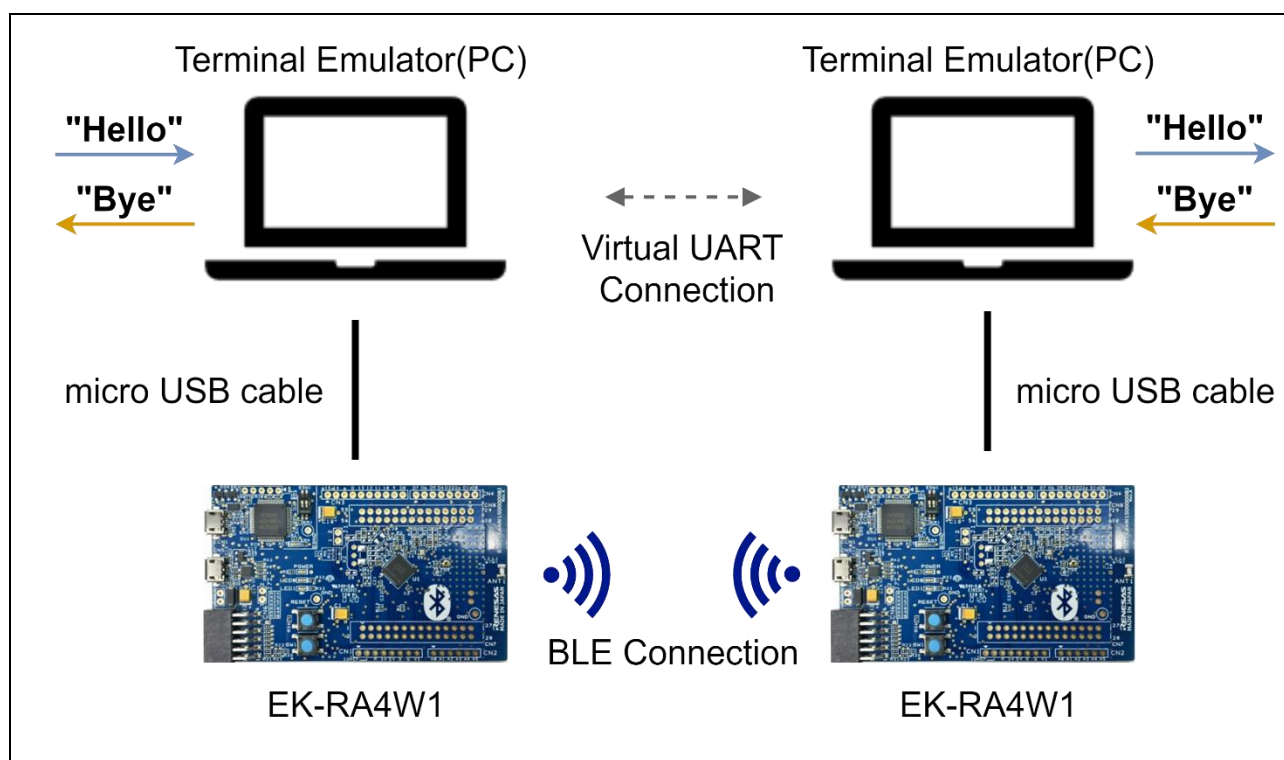
Figure 4. Operating environment of VUART App
