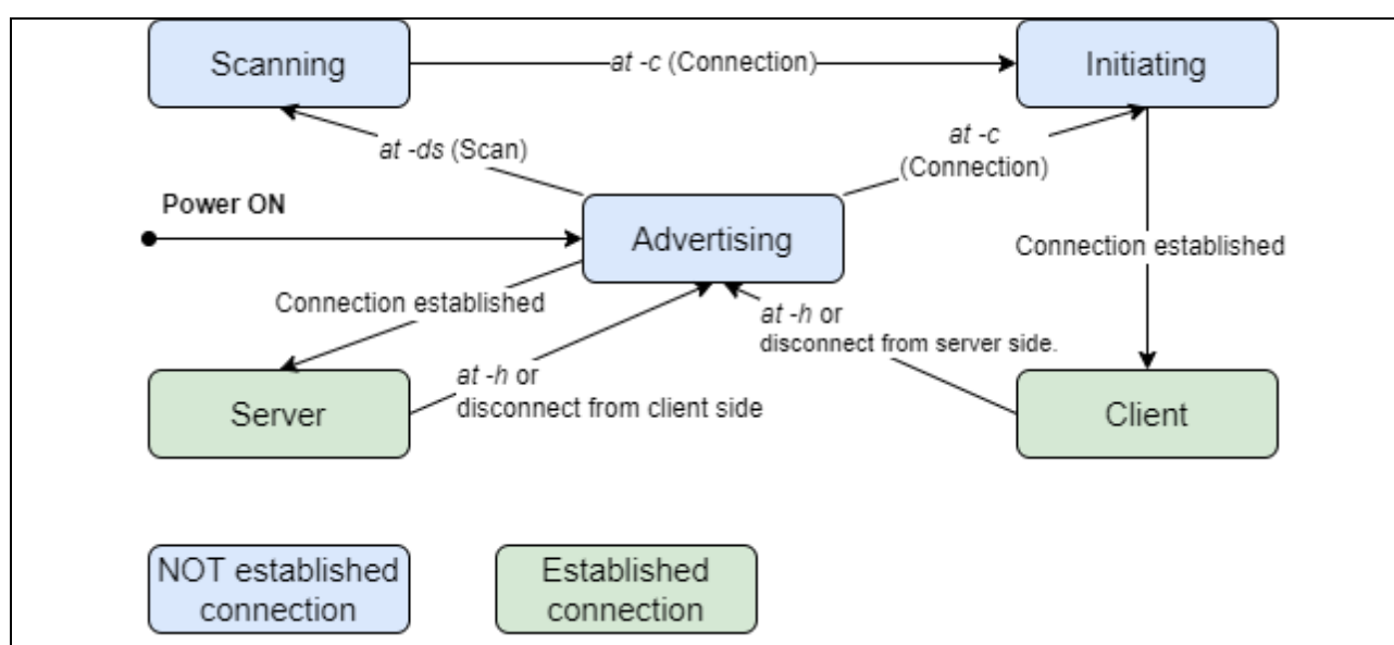
Figure 5. State transition diagram of the VUART App
