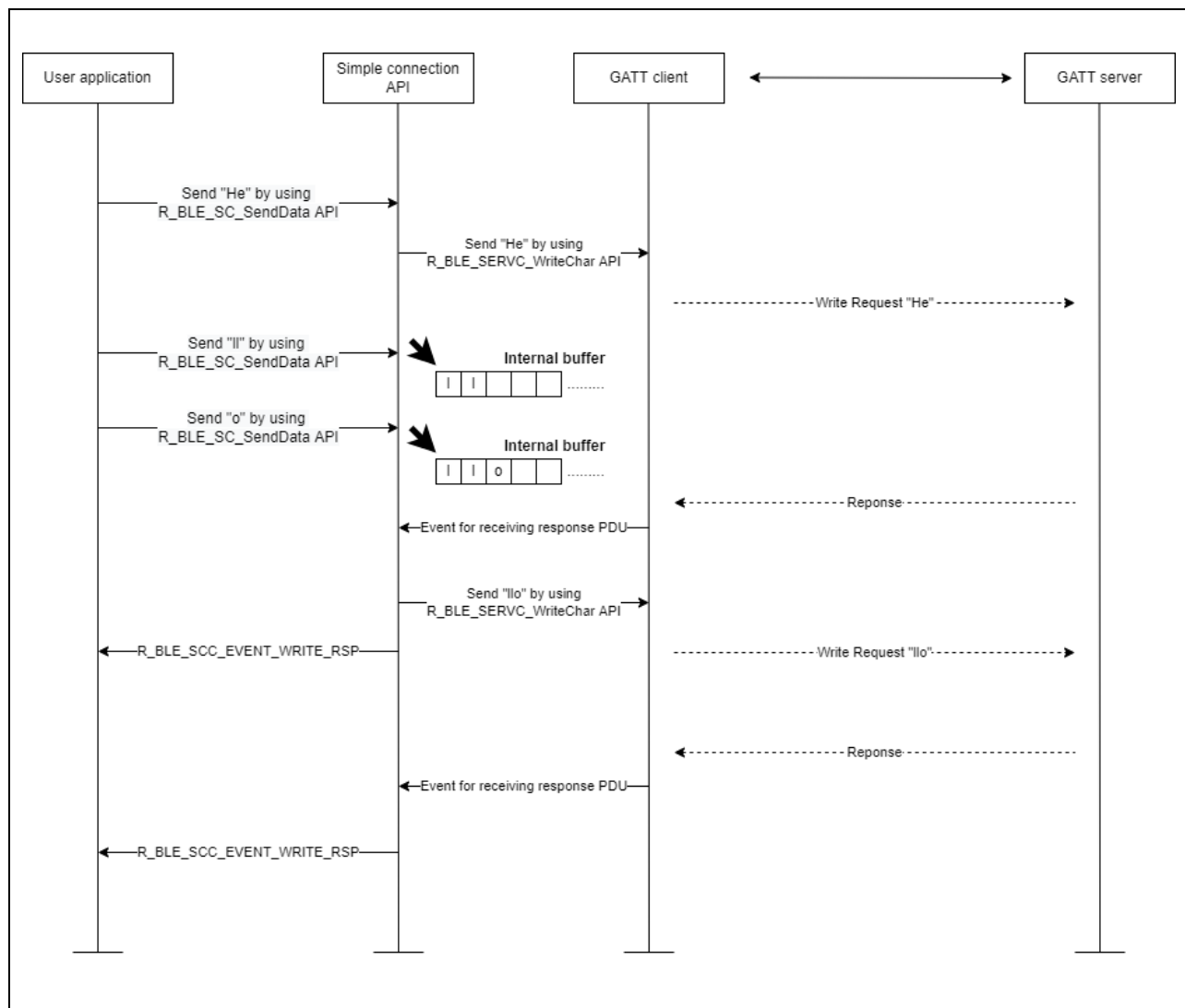
Figure 2. The behavior of the internal buffer
