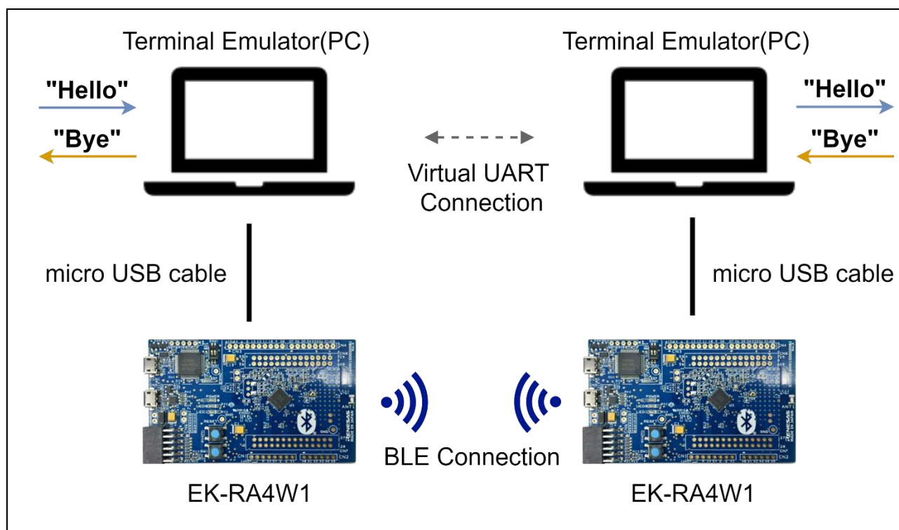
Figure 1. Operating environment of VUART App
