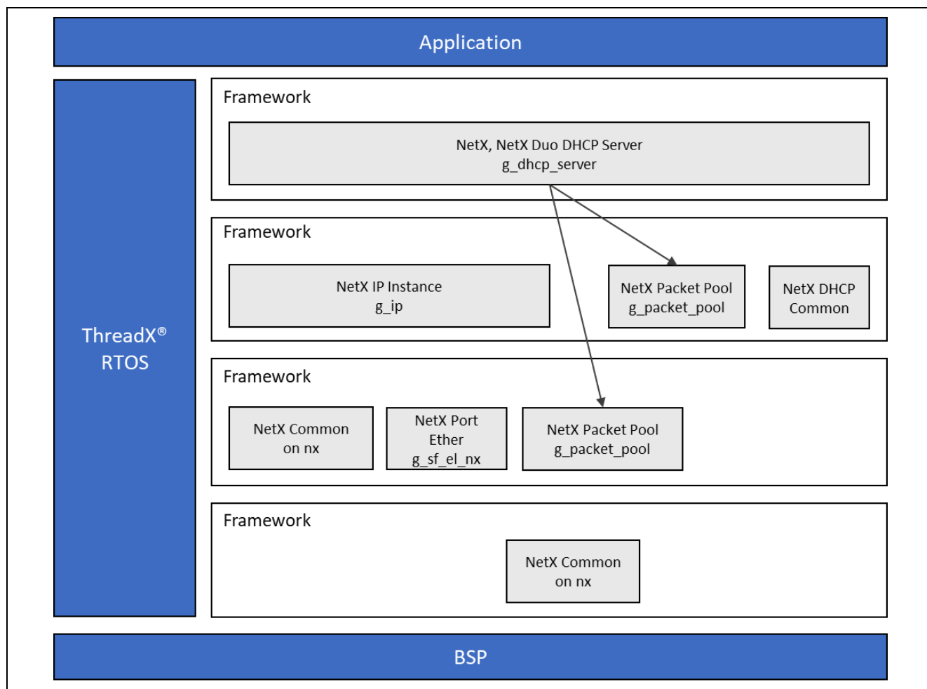
Figure 1. NetX DHCP Server Module Block Diagram
