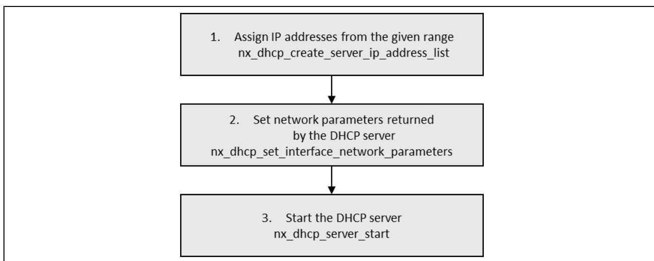
Figure 4. NetX DHCP Server Module Application Project Flow Diagram
