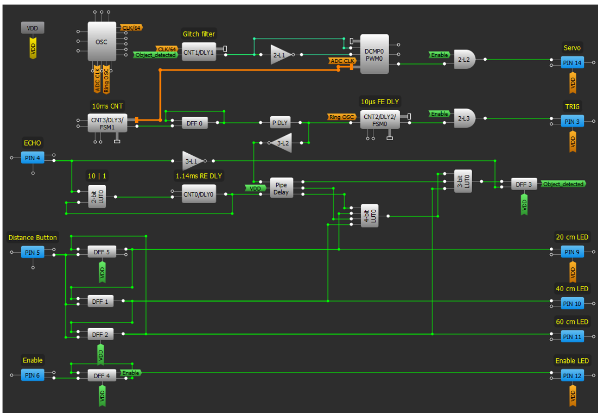
Figure 2: GreenPAK Design
