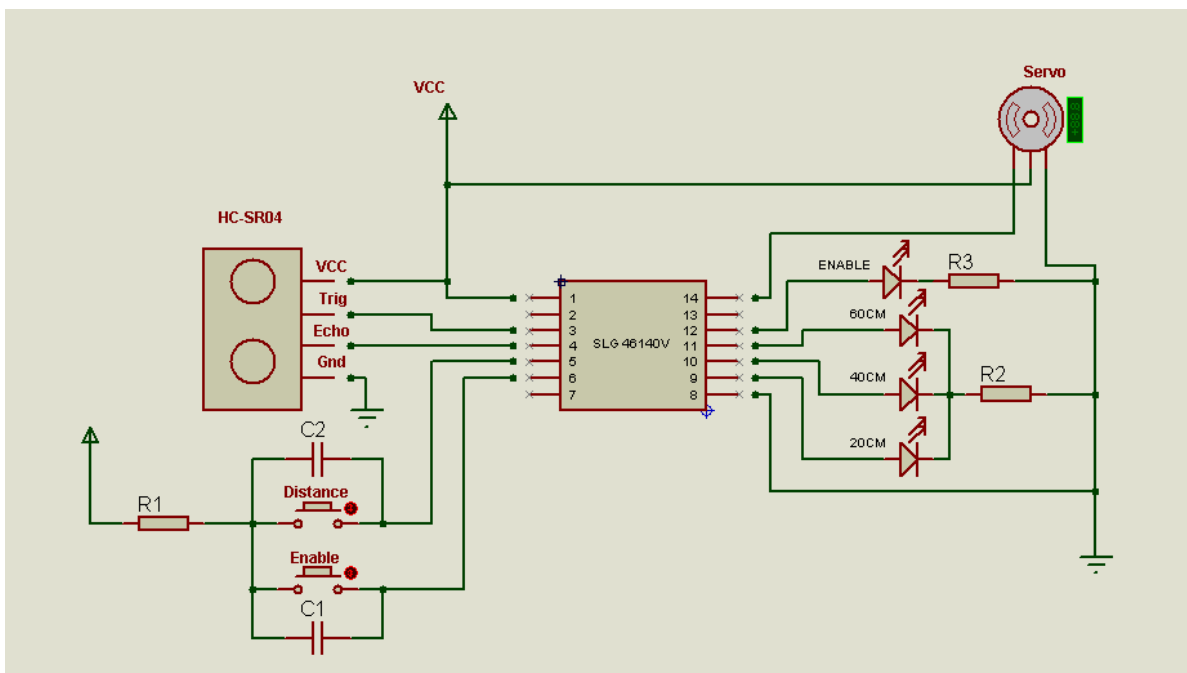
Figure 3: Top Level Circuit Diagram
