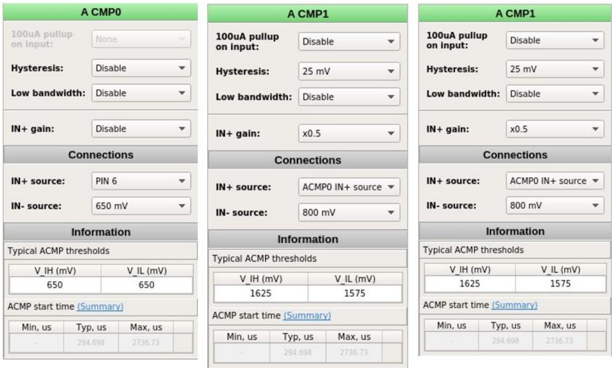
Figure 11: ACMP's Settings
