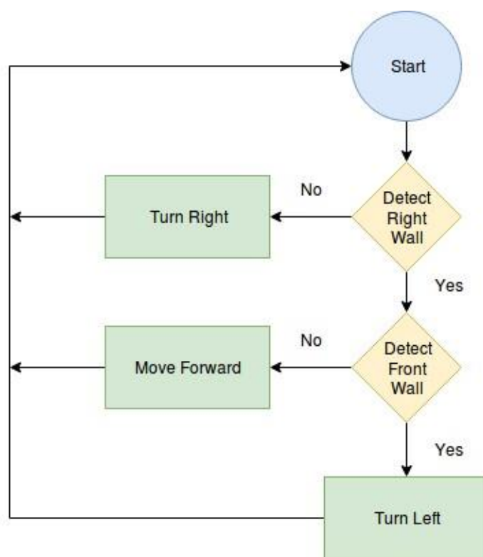
Figure 7: Simplified Algorithm
