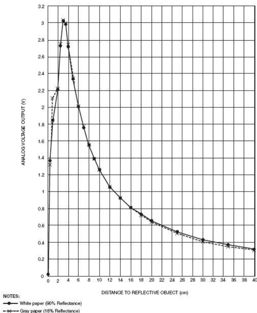
Figure 1: Distance-Voltage Graph
