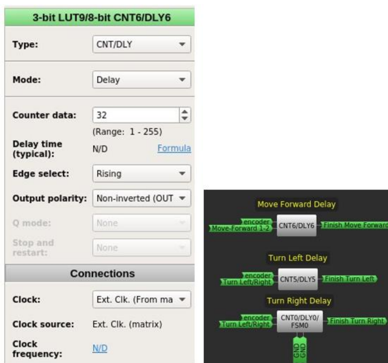
Figure 15: Move Forward Delay Settings and Circuits
