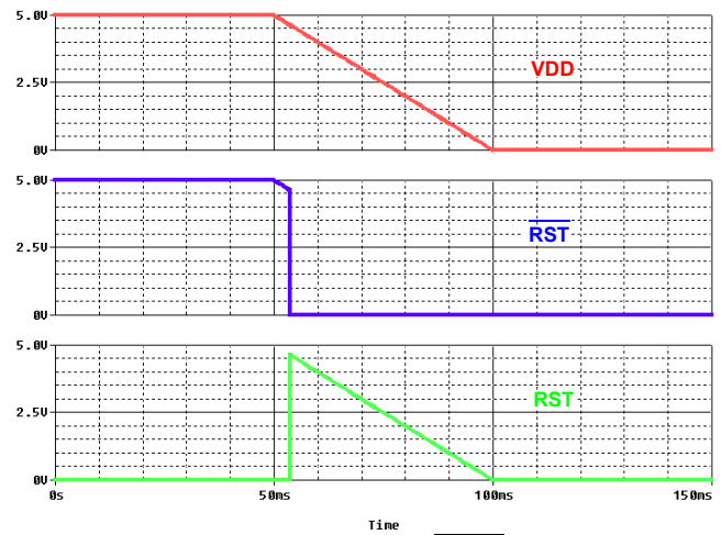
FIGURE 3. ISL705xRH RESET and \overline{\text{RESET}} DEASSERTION
