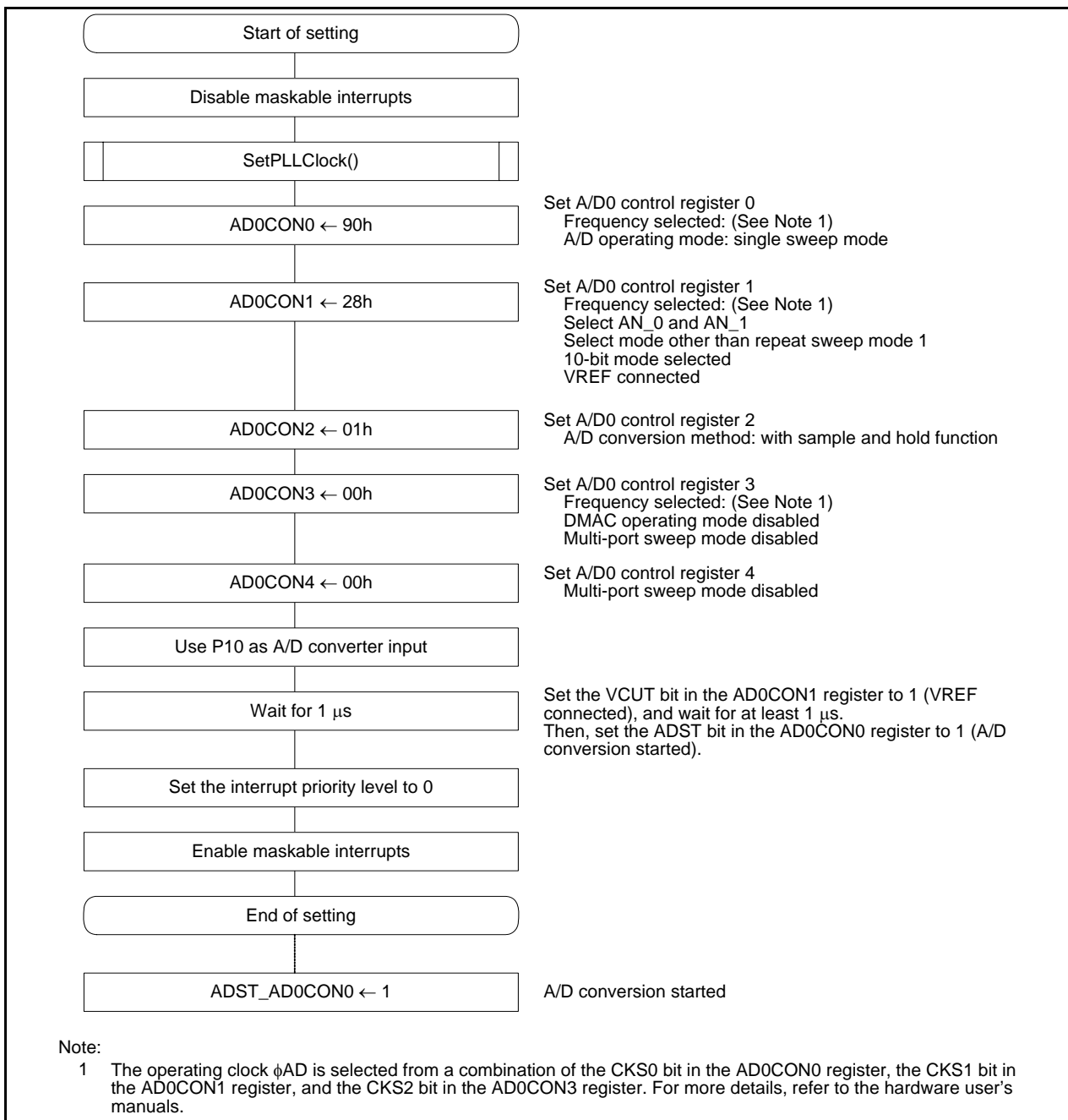
Figure 3.2 Setting Procedure of Single Sweep Mode
