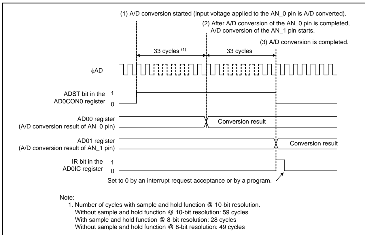
Figure 3.1 Operation Example in Single Sweep Mode
