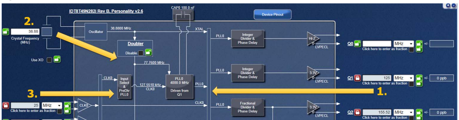
Figure 1. Jitter Attenuator vs Synthesizer Mode
