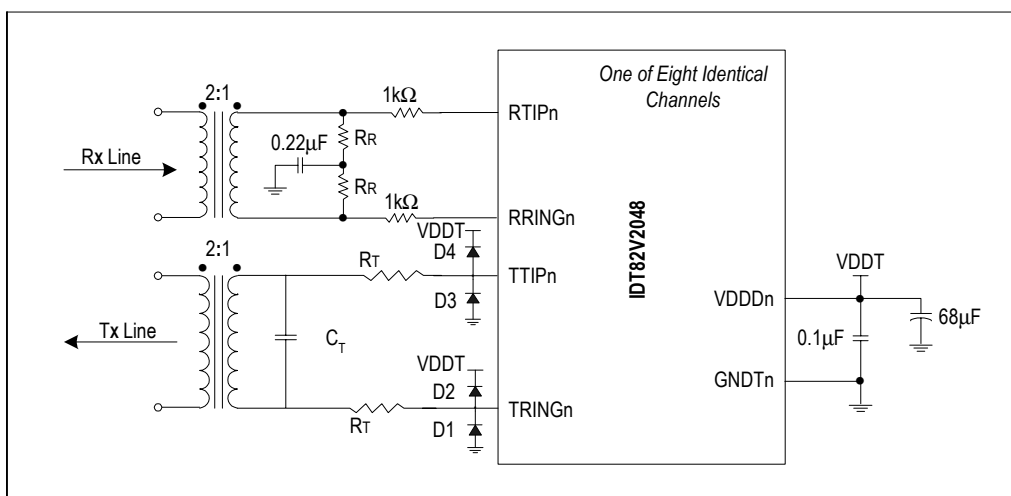
Figure 1. Recommended Application Circuit
