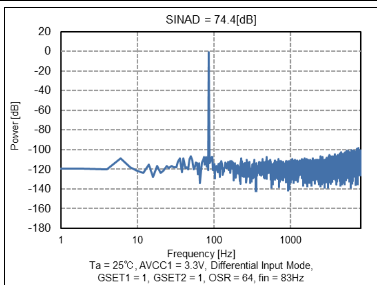
図 13 周波数と出力の対比 ( G_{SET1} = 1 , G_{SET2} = 1 , OSR = 64 )
