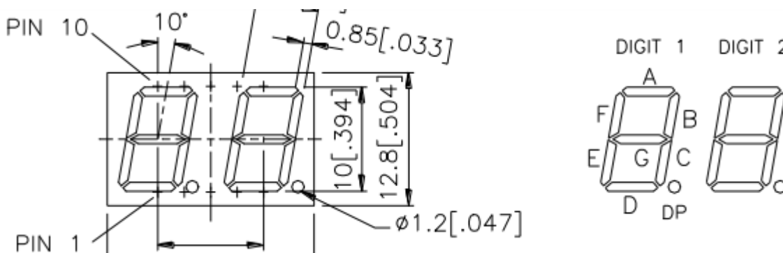
Figure 8. LTD-4708JF display
