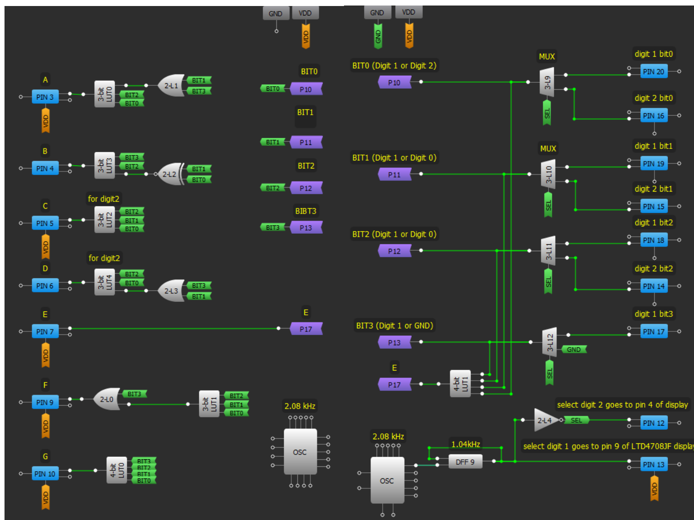
Figure 11. GreenPAK Design
