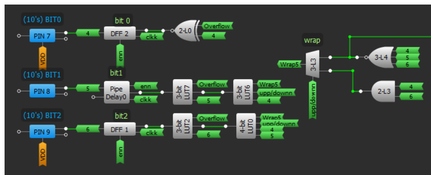
Figure 2. 10s digit counter (Matrix 1)
