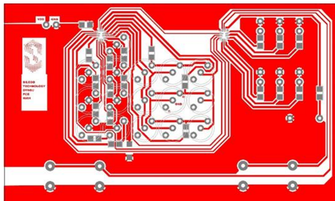
Figure 6. Dino Game PCB layout
