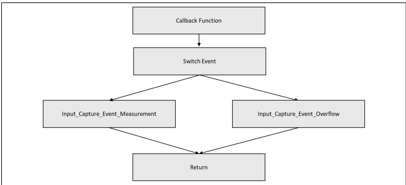
Figure 5. Detailed flow chart of callback function
