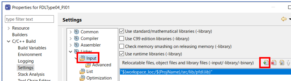
Figure 6-17 (a). Specifying the Library File (CC-RL)
