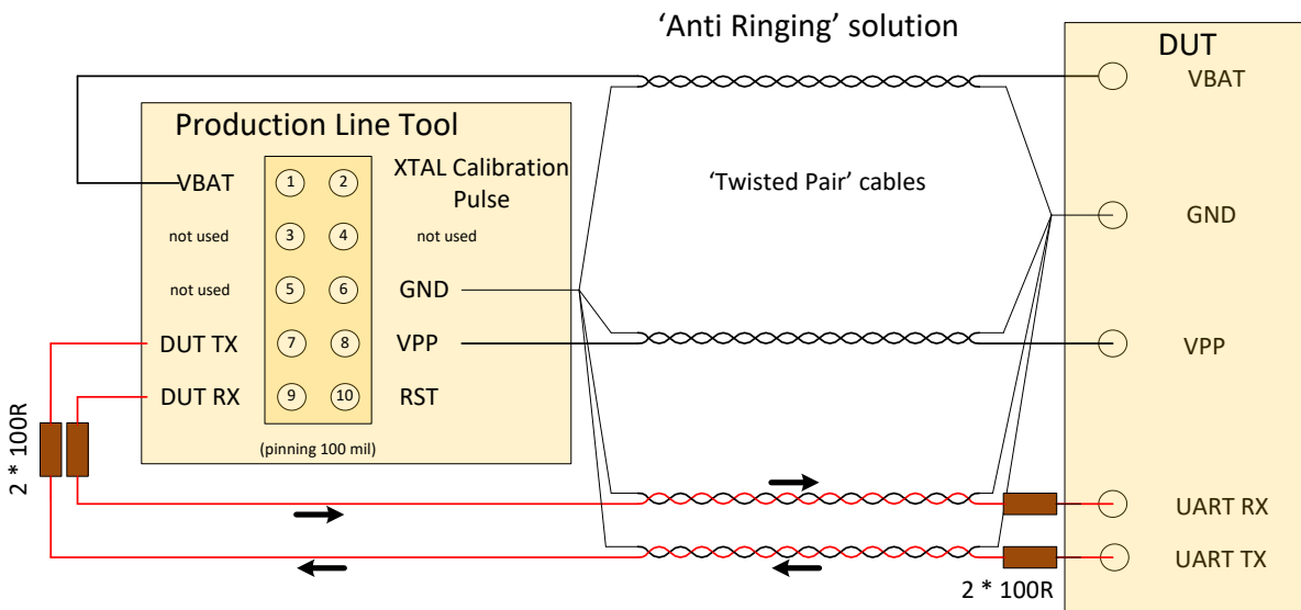
Figure 166: Anti-Ringing Solution
