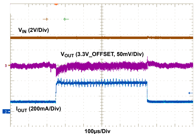
Figure 50. Load Transient: V_{IN} = 3.6V , V_{OUT} = 3.3V , Load = 0.125A to 0.375A, Slew Rate = 1A/ \mu s
