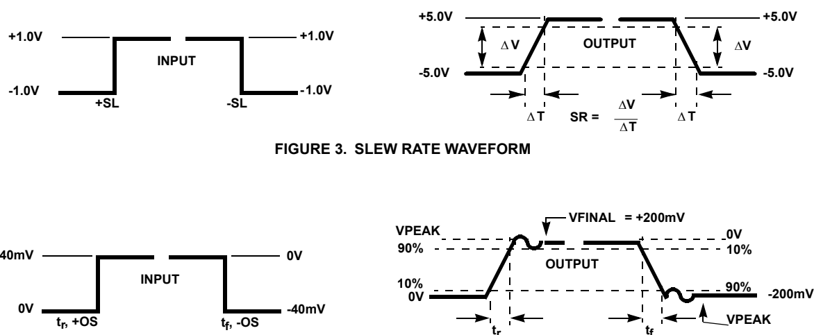
FIGURE 4. OVERSHOOT, RISE AND FALL TIME WAVEFORMS
