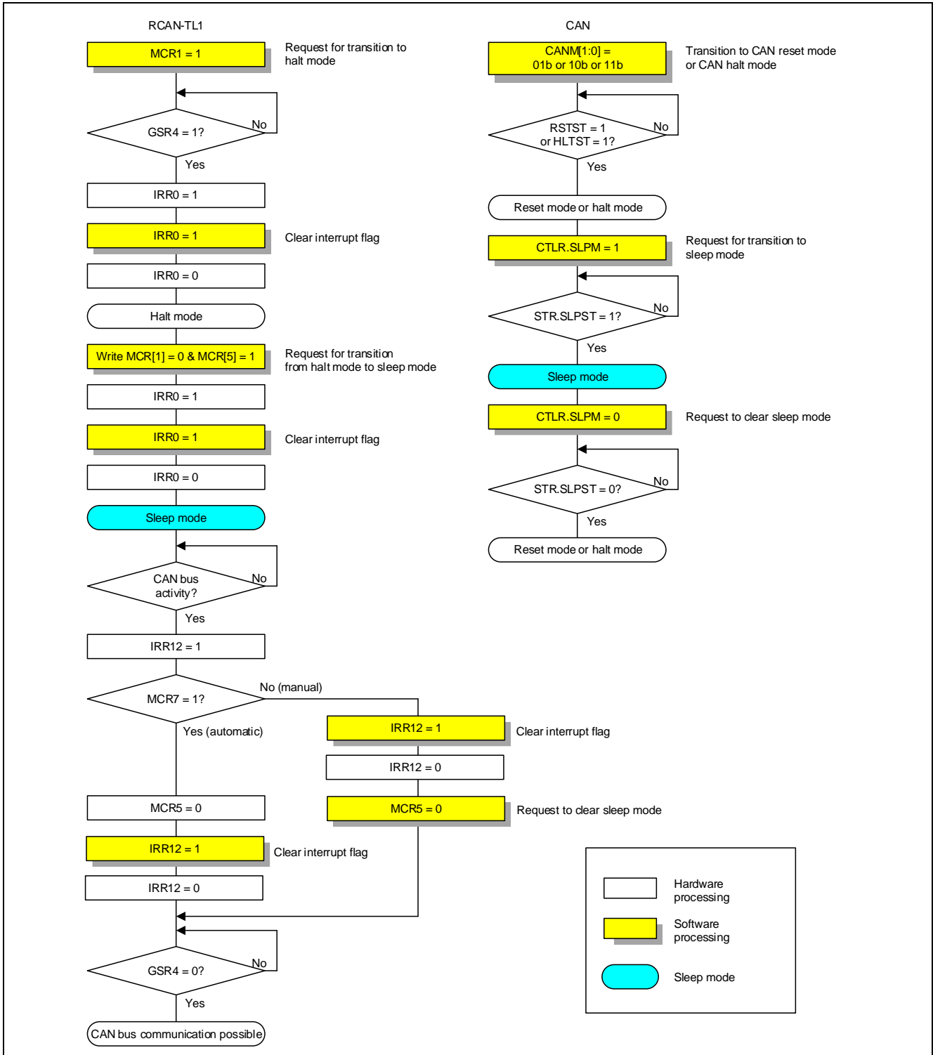
Figure 4.1 Sleep Mode Setting Procedure on H8SX/1720S (RCAN-TL1) and RX65N (CAN)
