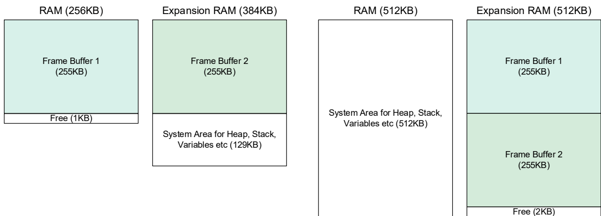
Figure 1.4 Example of Frame Buffer Allocation
