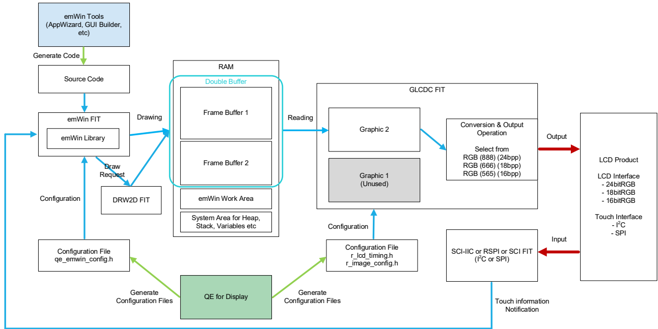
Figure 1.2 RGB (Parallel Interface) Configuration
