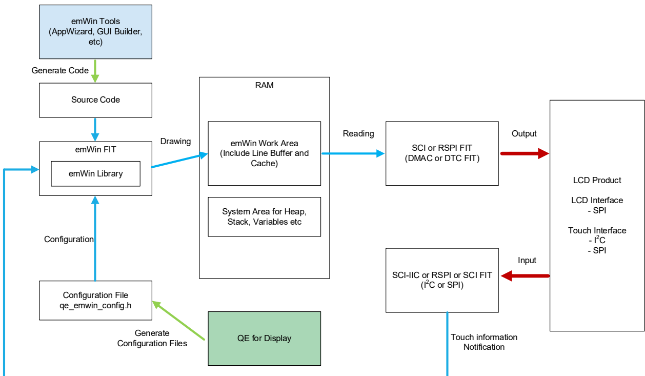
Figure 1.3 SPI (Serial Interface) Configuration
