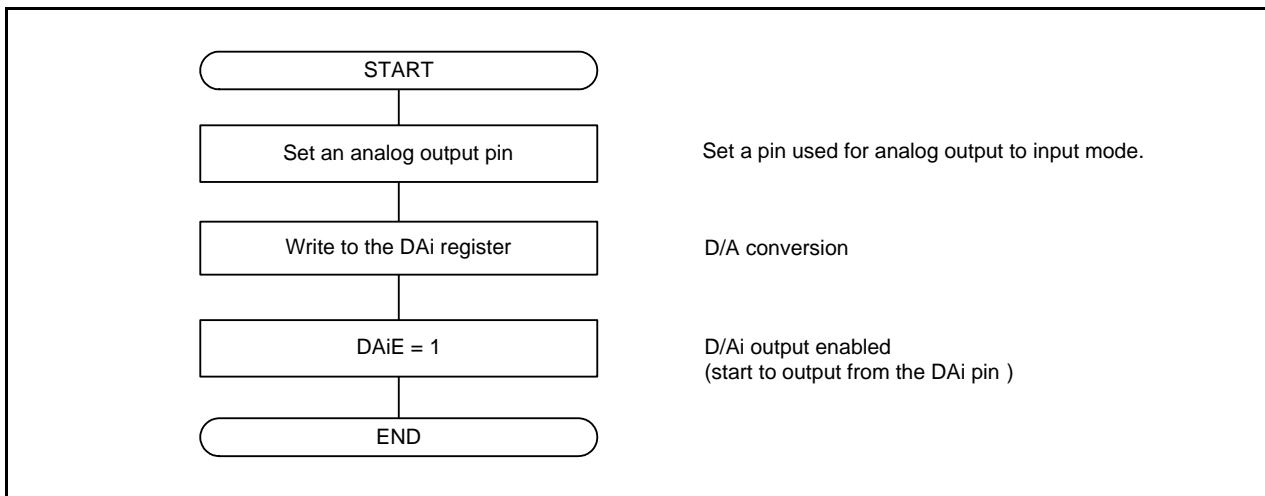
Figure 4.1 D/A Output Operation Procedure ( i = 0, 1 )
