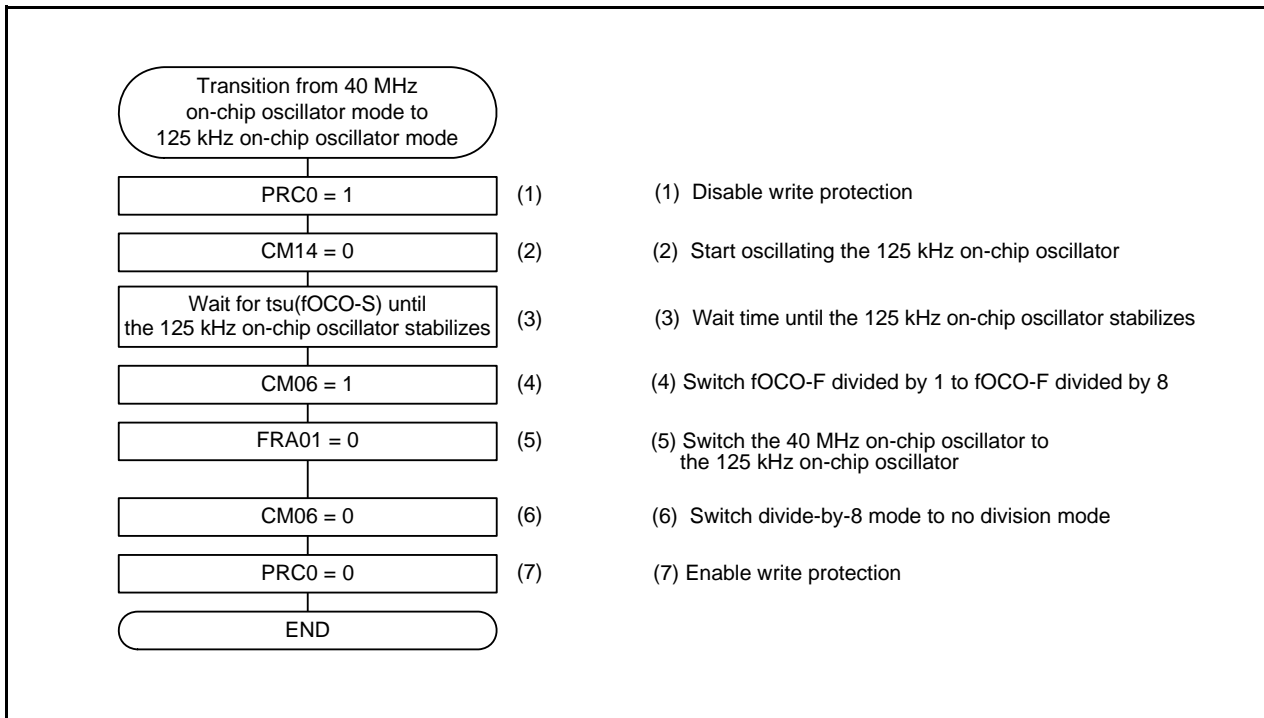
Figure 3.2 Transition from 40 MHz On-Chip Oscillator Mode (fOCO-F Divided by 1) to 125 kHz On-Chip Oscillator mode
