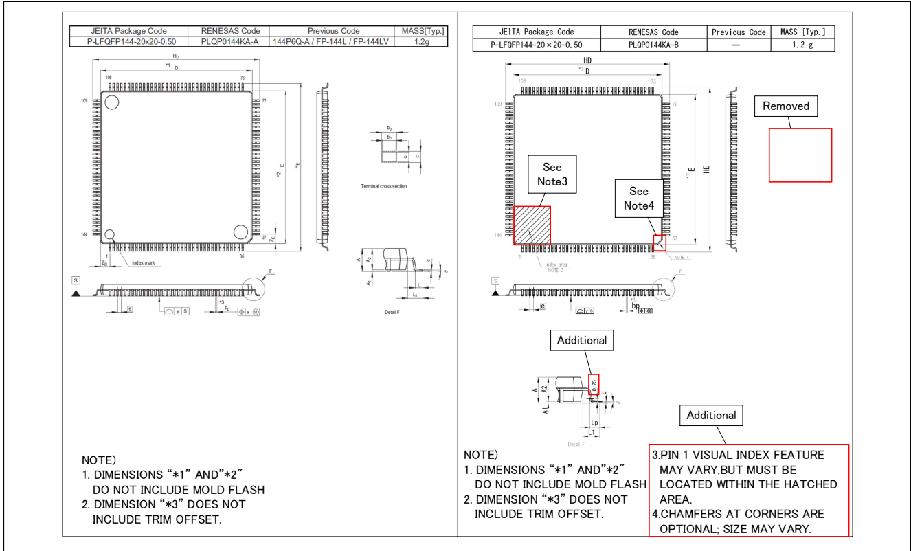
Figure 2.1 Differences in external form for QFP-144pin
