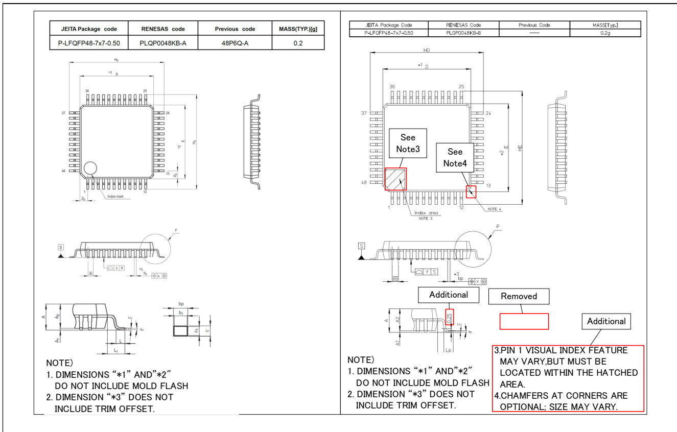
Figure 2.6 Differences in external form for QFP-48pin
