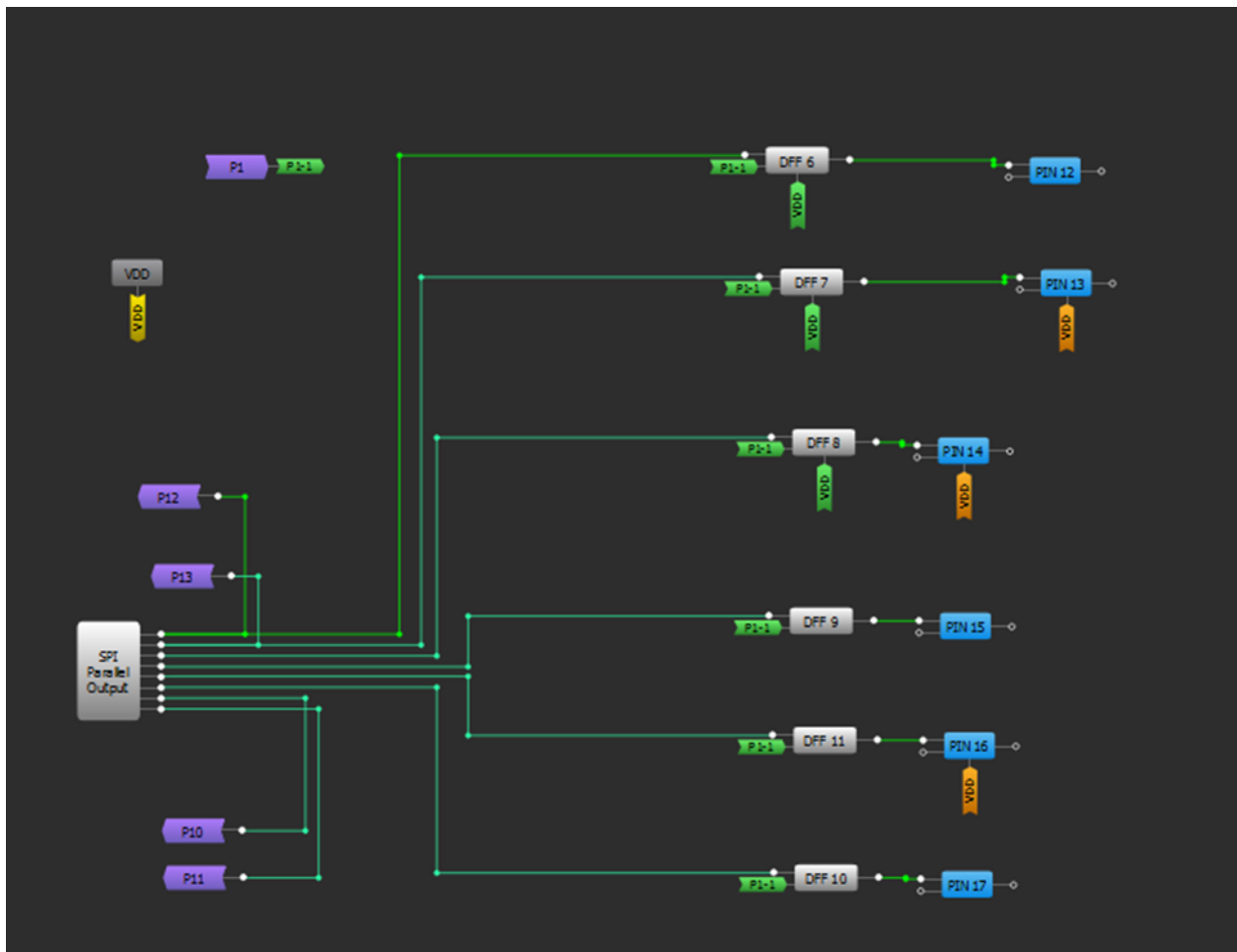
Figure 5. SPI Parallel Output Block Pins
