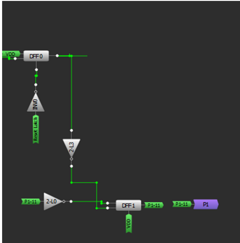
Figure 6. Mod 2 Counter for data Parsing
