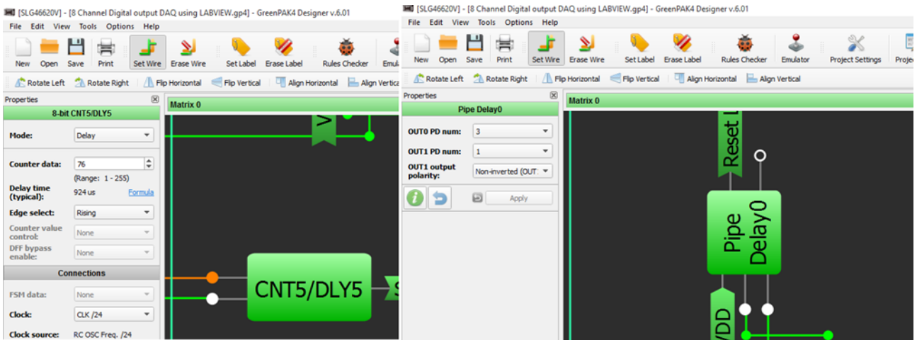
Figure 4. CNT5/DLY5 and Pipe Delay 0 properties
