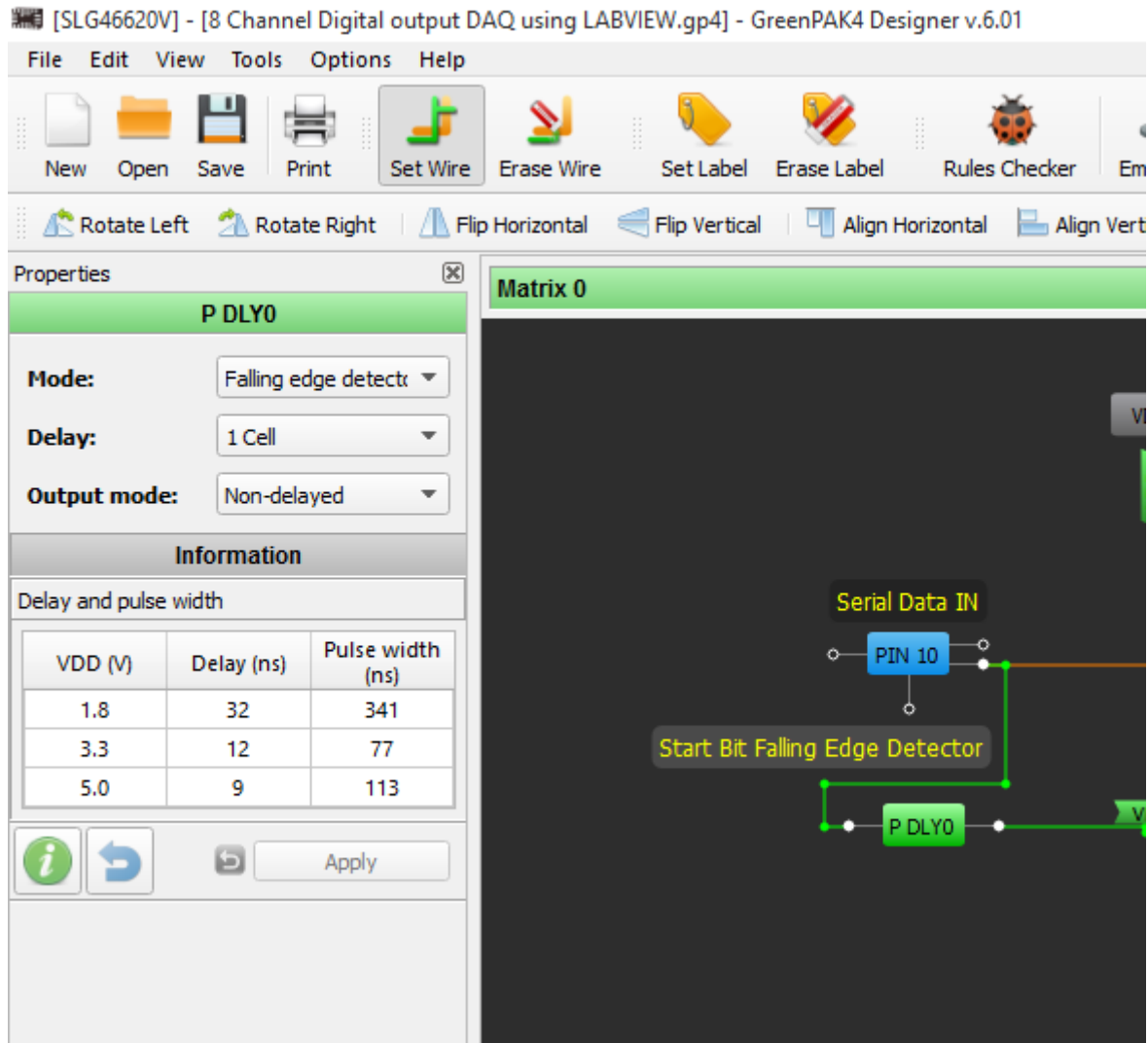
Figure 3. P DLY0 block Properties
