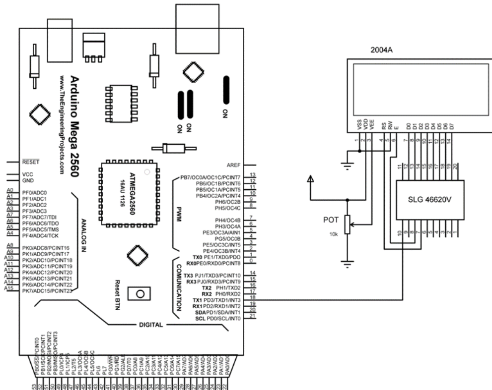
Figure 1. Hardware Schematic
