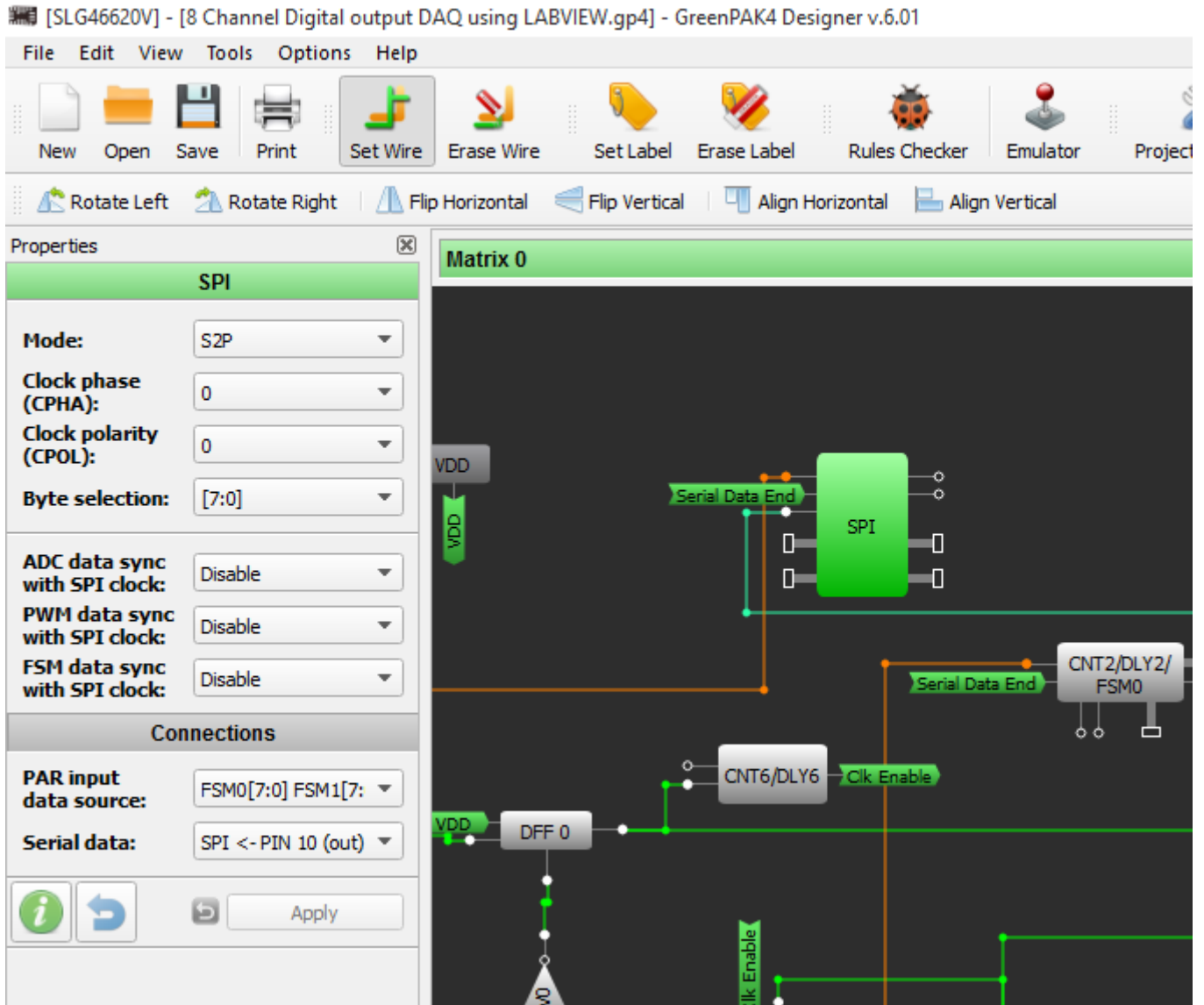
Figure 2. Serial Data received in GreenPAK
