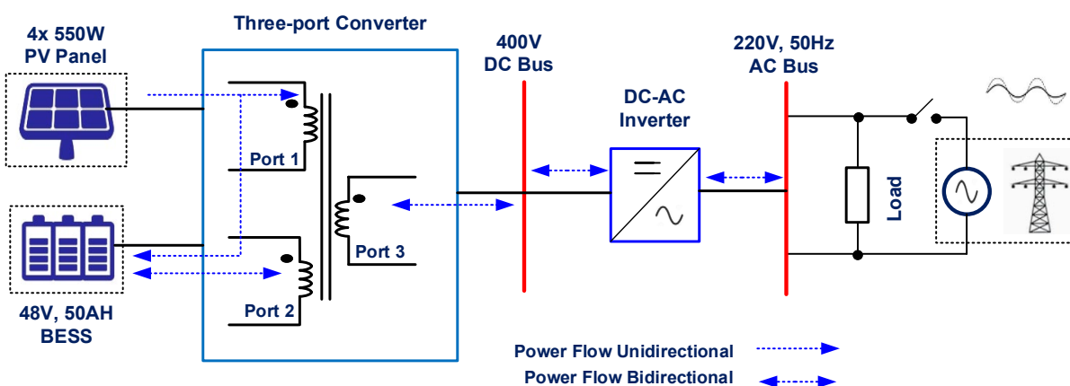
Fig.3 Multiport Architecture
