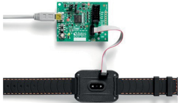
Figure 17: Wearable Device with Associated Interface Board
