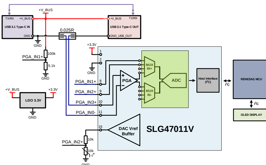
Figure 4. Functional Block Diagram of SLG47011V Demo Board #1 R1.0
