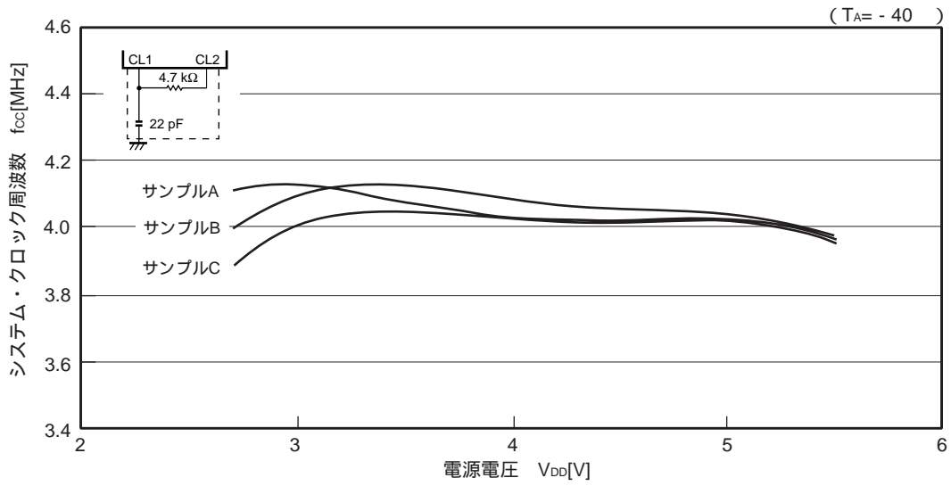
f cc vs V DD (RC発振, R = 4.7 kΩ, C = 22 pF)
