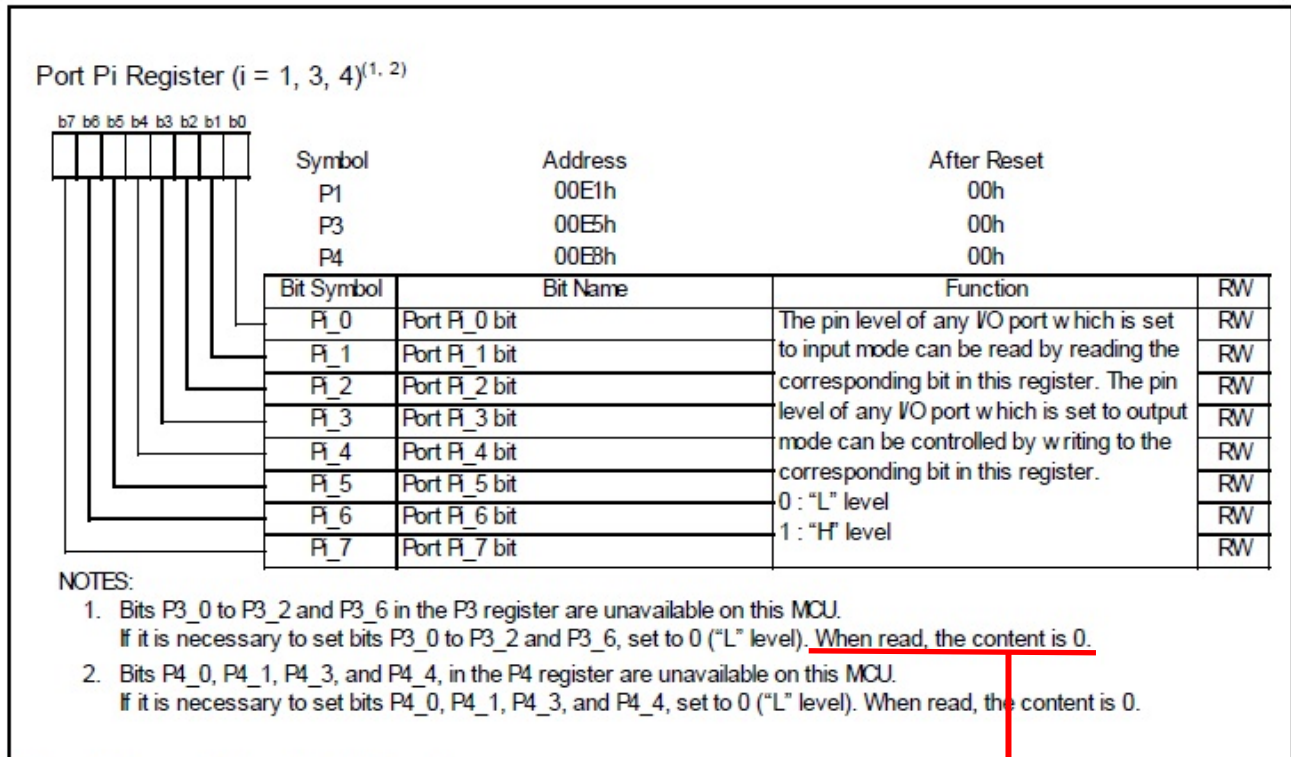
Figure 7.7 Pi ( i = 1, 3, 4 ) Register
