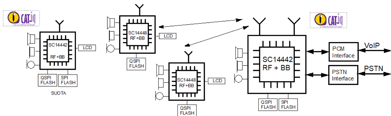
Figure 1. System diagram
