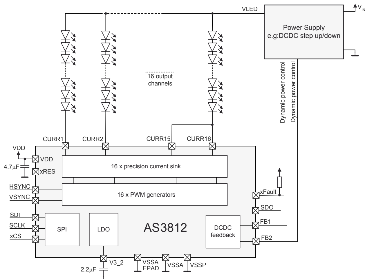
Figure 1. AS3812 Typical Application (With CURR15 and CURR16 connected together to show increased LED string current capability by paralleling outputs)
